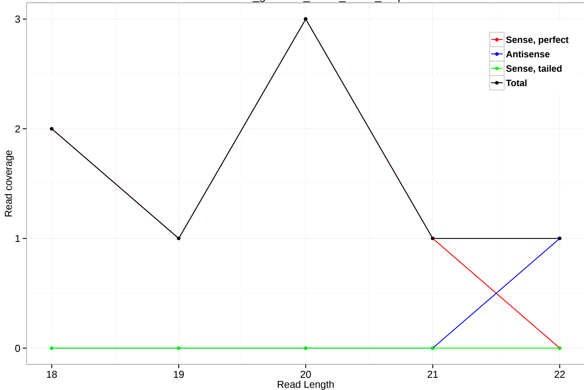
rheMac3_genscan_chr13_58.25_0.5p
