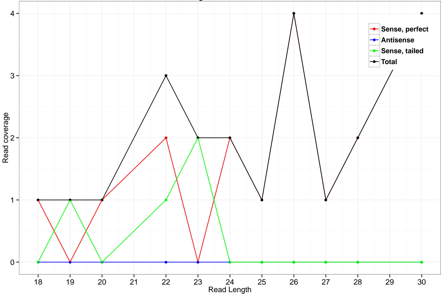
rheMac3_genscan_chr13_58.12_10
