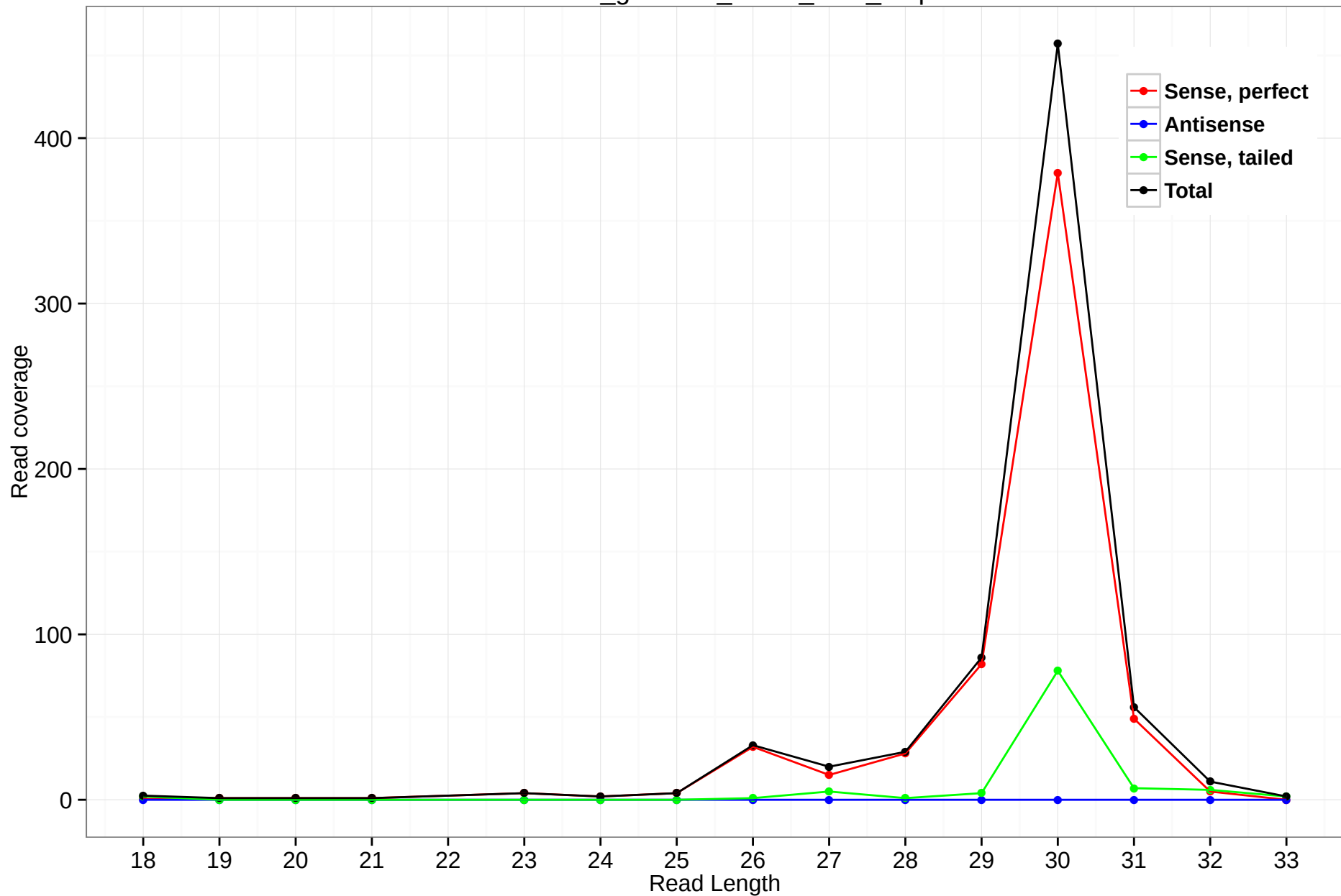
rheMac3_genscan_chr13_57.3_1.3p
