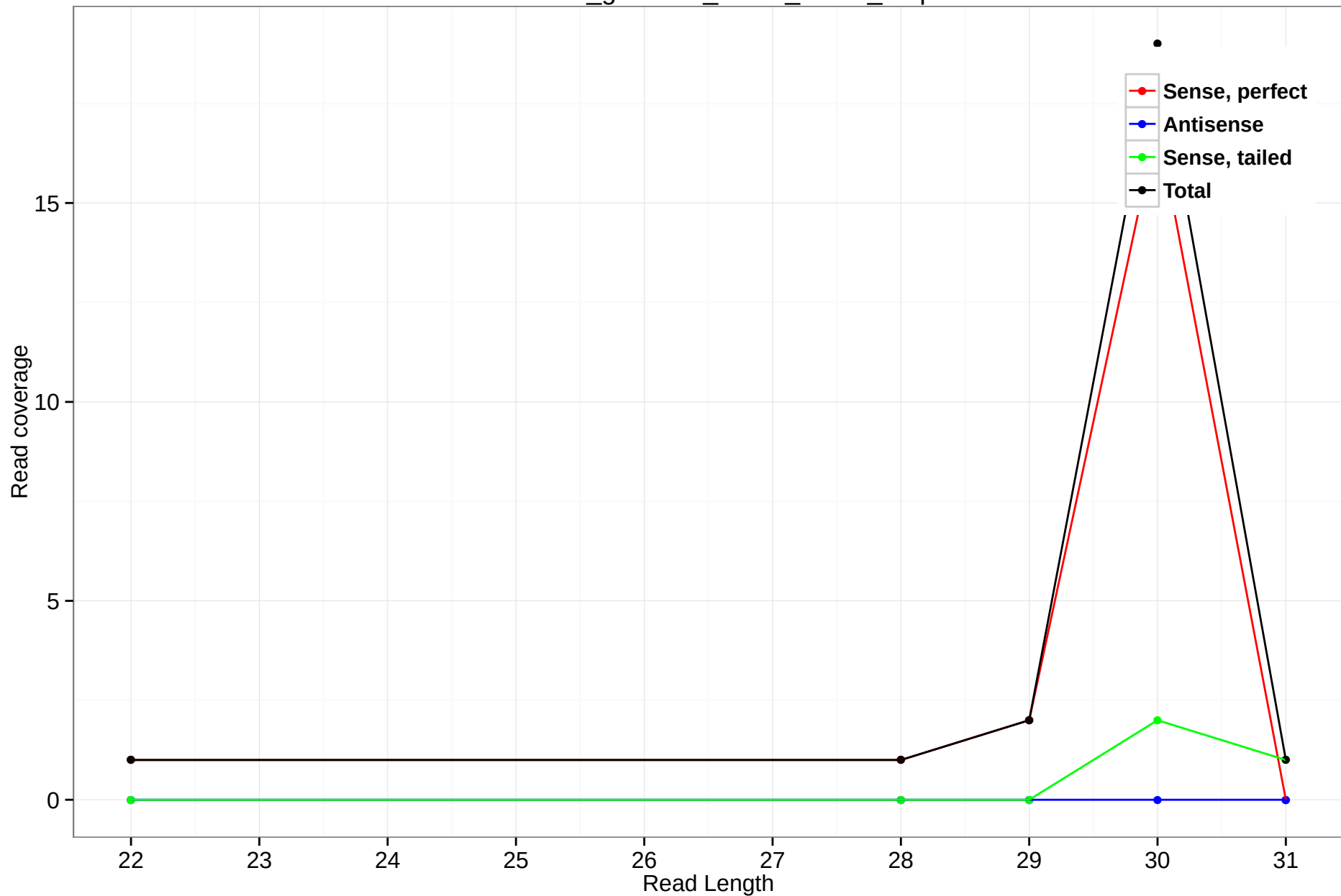
rheMac3_genscan_chr13_57.14_7.5p
