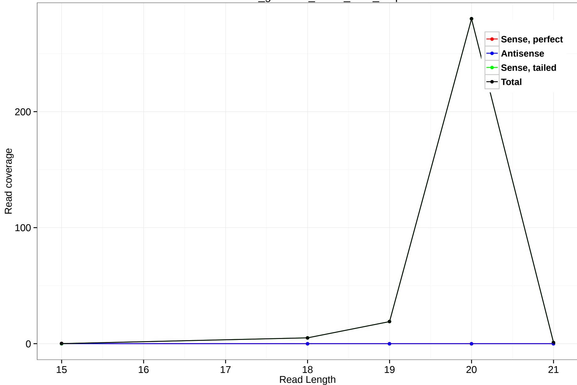
rheMac3_genscan_chr13_56.6_5.3p
