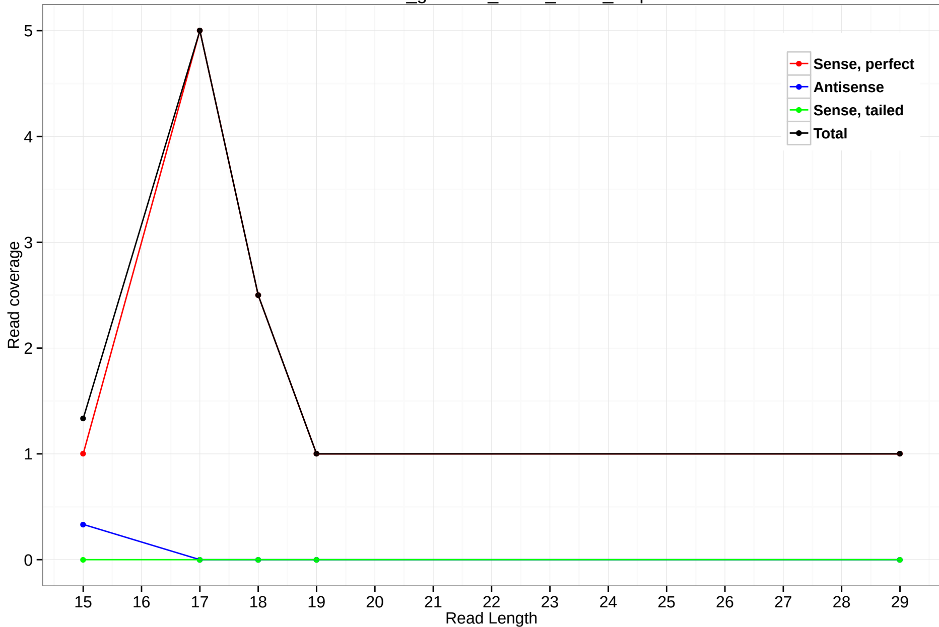
rheMac3_genscan_chr13_55.63_6.5p
