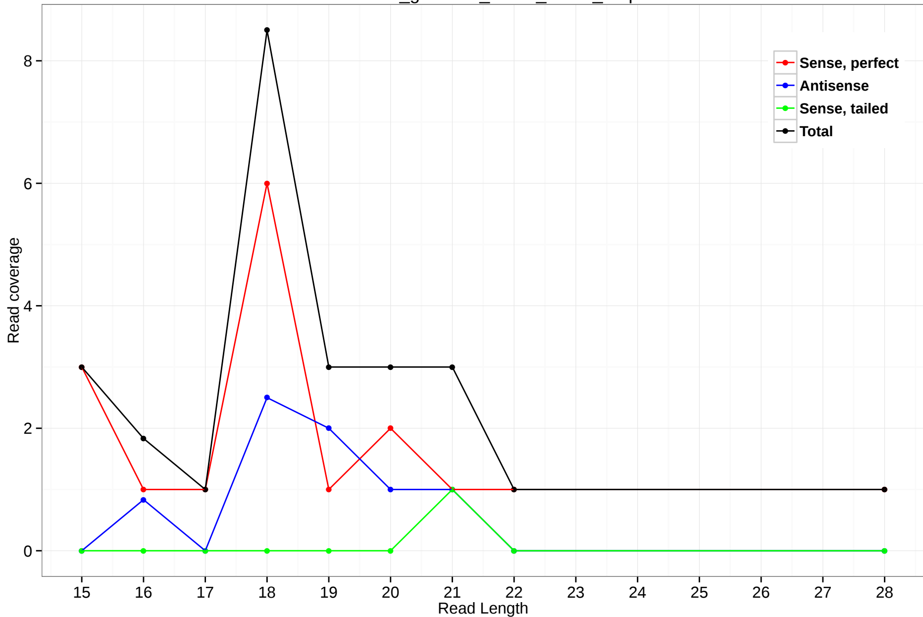
rheMac3_genscan_chr13_55.21_9.5p
