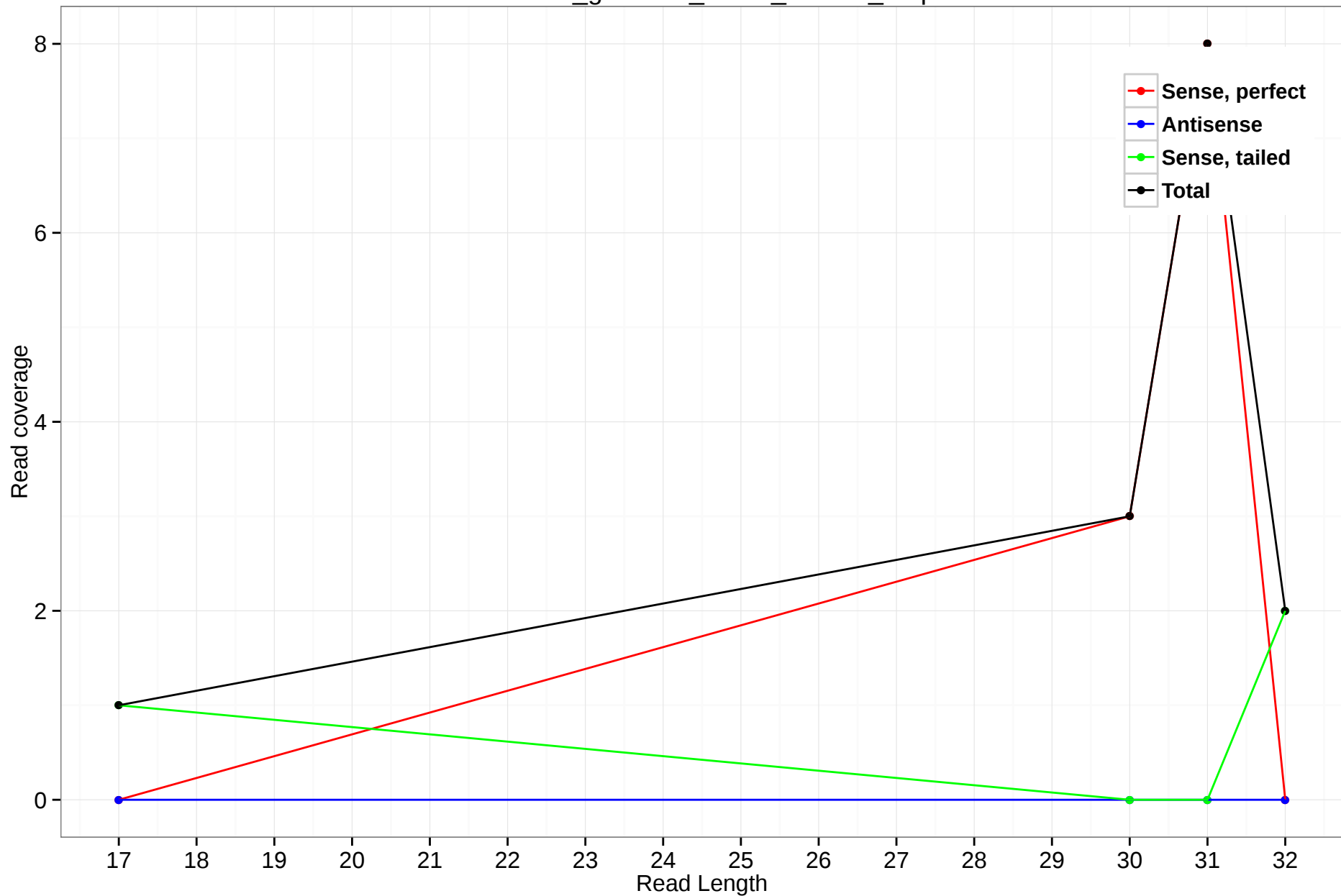
rheMac3_genscan_chr13_55.129_5.5p
