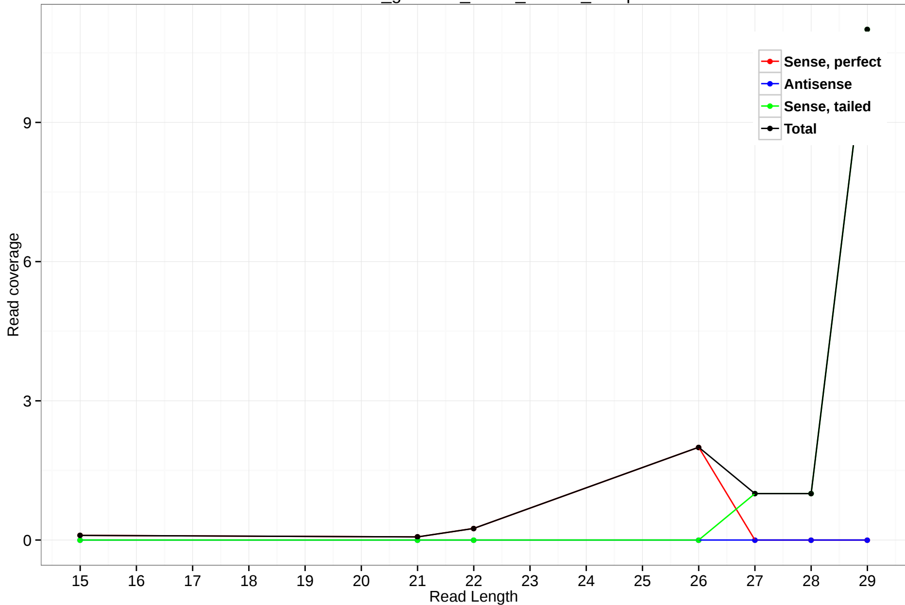
rheMac3_genscan_chr13_55.112_10.5p
