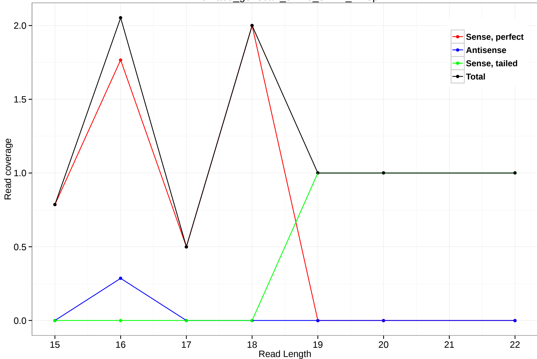
rheMac3_genscan_chr13_54.22_21.5p
