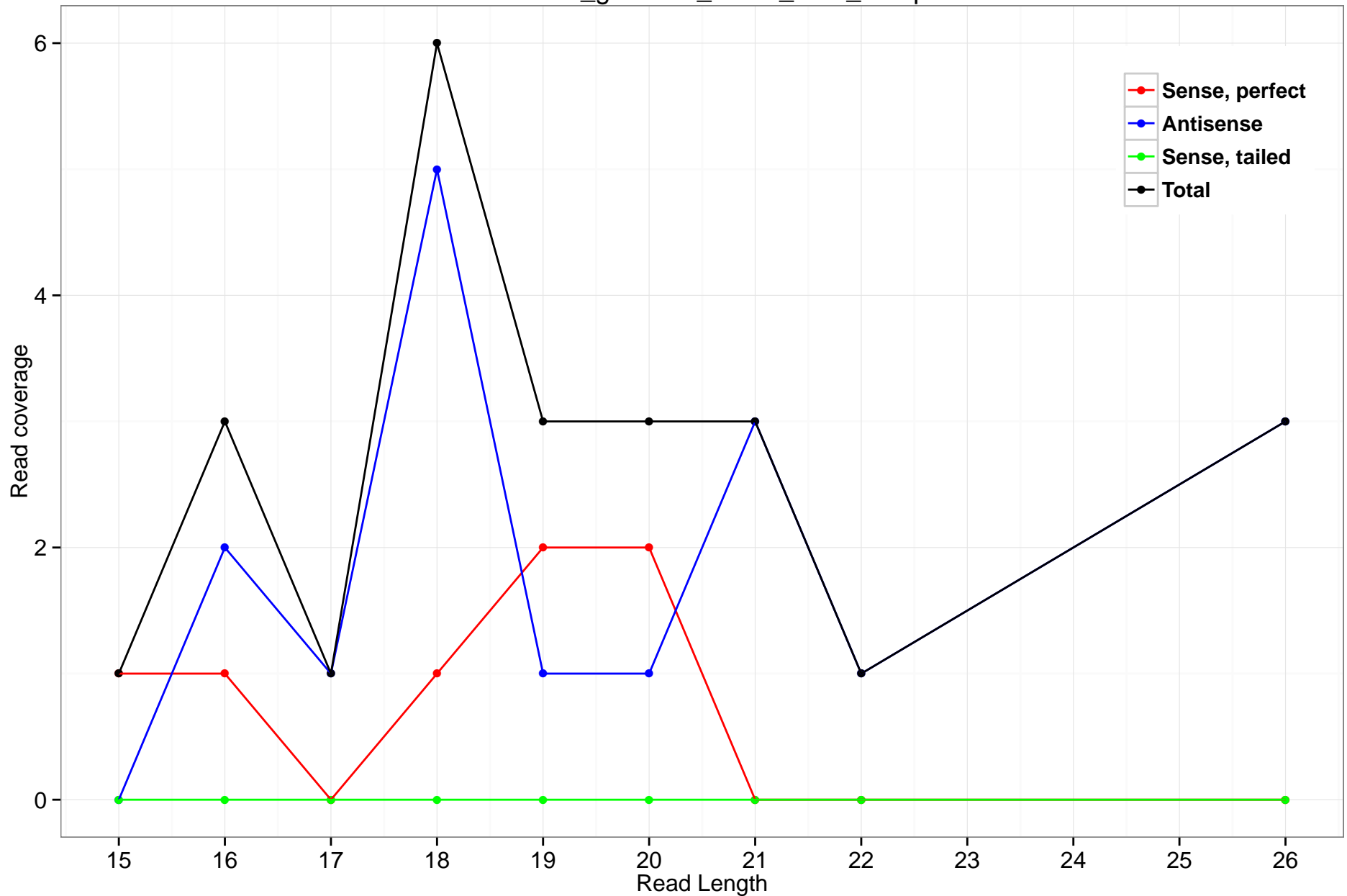
rheMac3_genscan_chr13_52.9_21.5p
