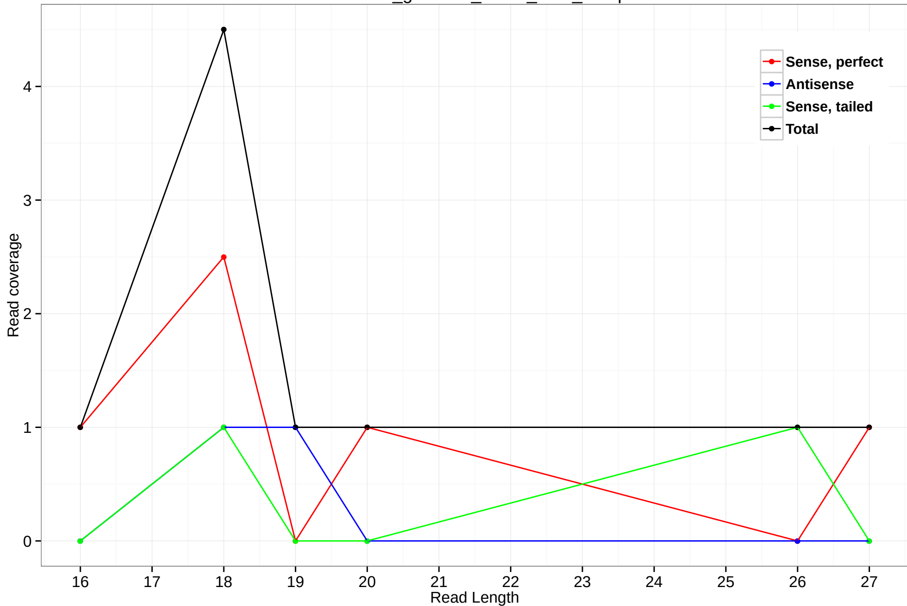
rheMac3_genscan_chr13_52.9_21.3p
