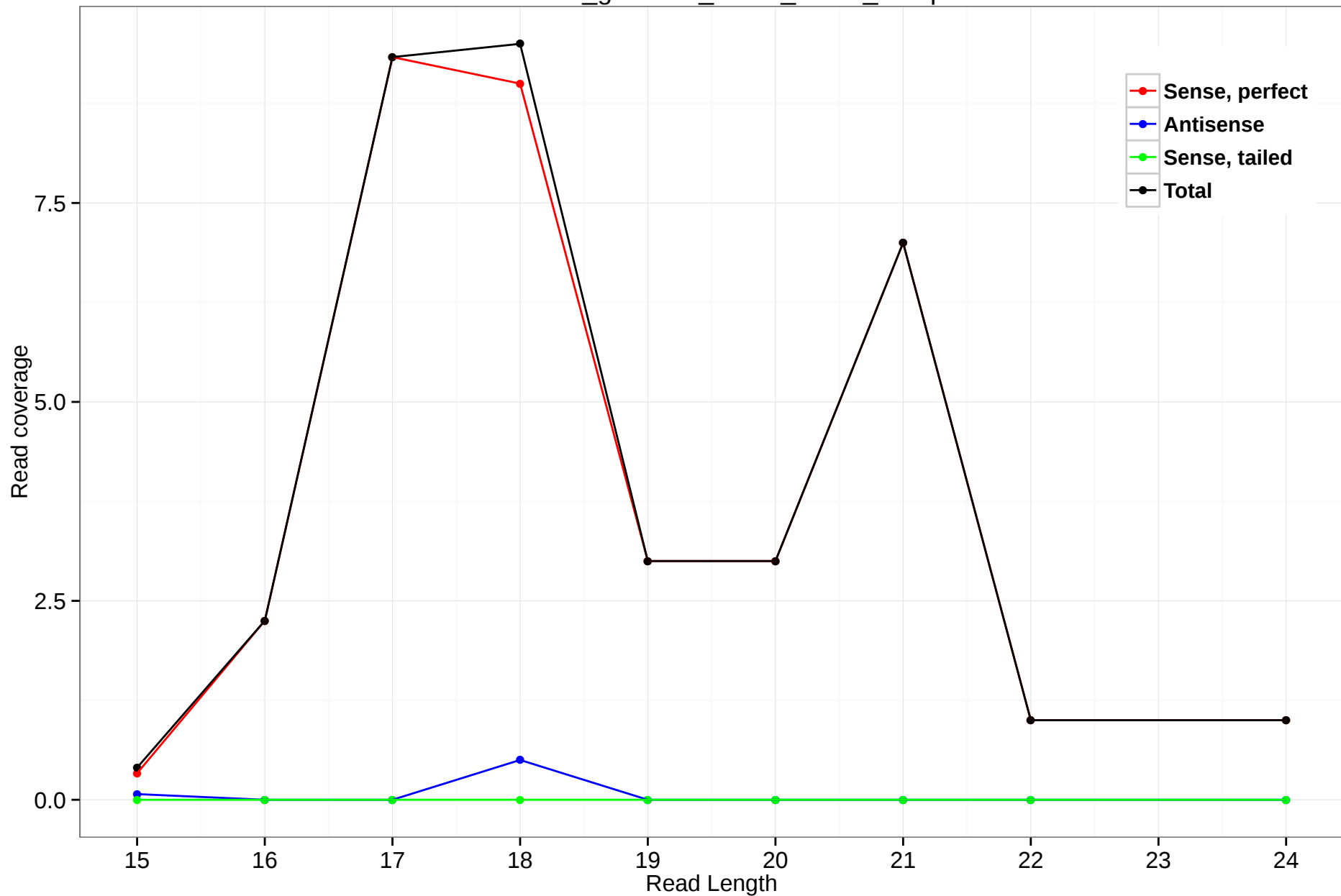
rheMac3_genscan_chr13_51.21_11.3p
