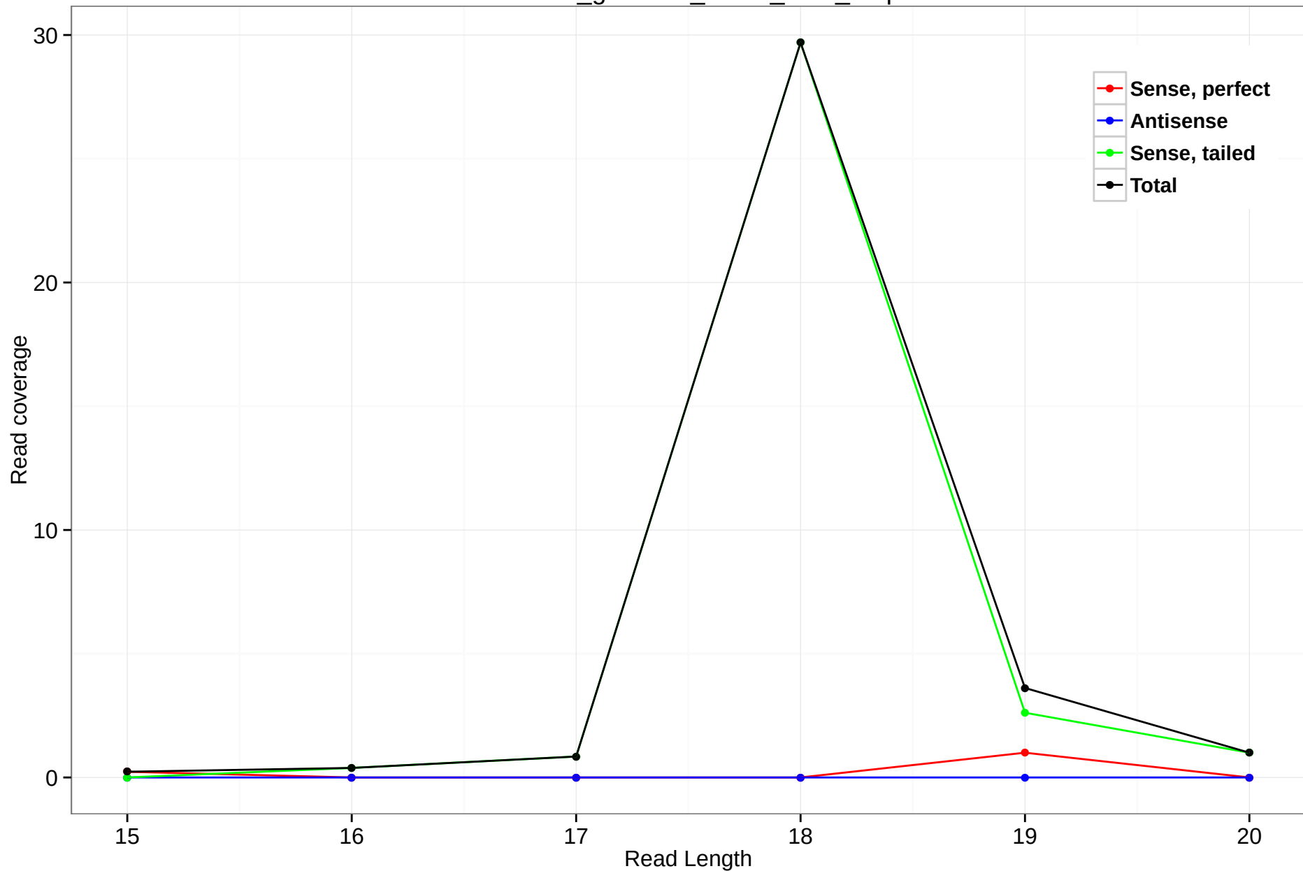
rheMac3_genscan_chr13_48.3_3.5p
