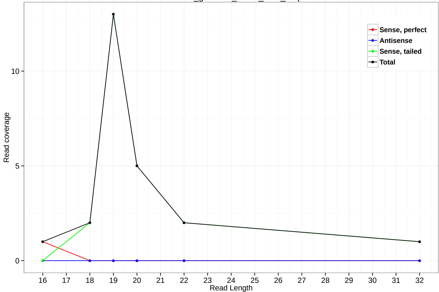
rheMac3_genscan_chr13_40.9_2.3p
