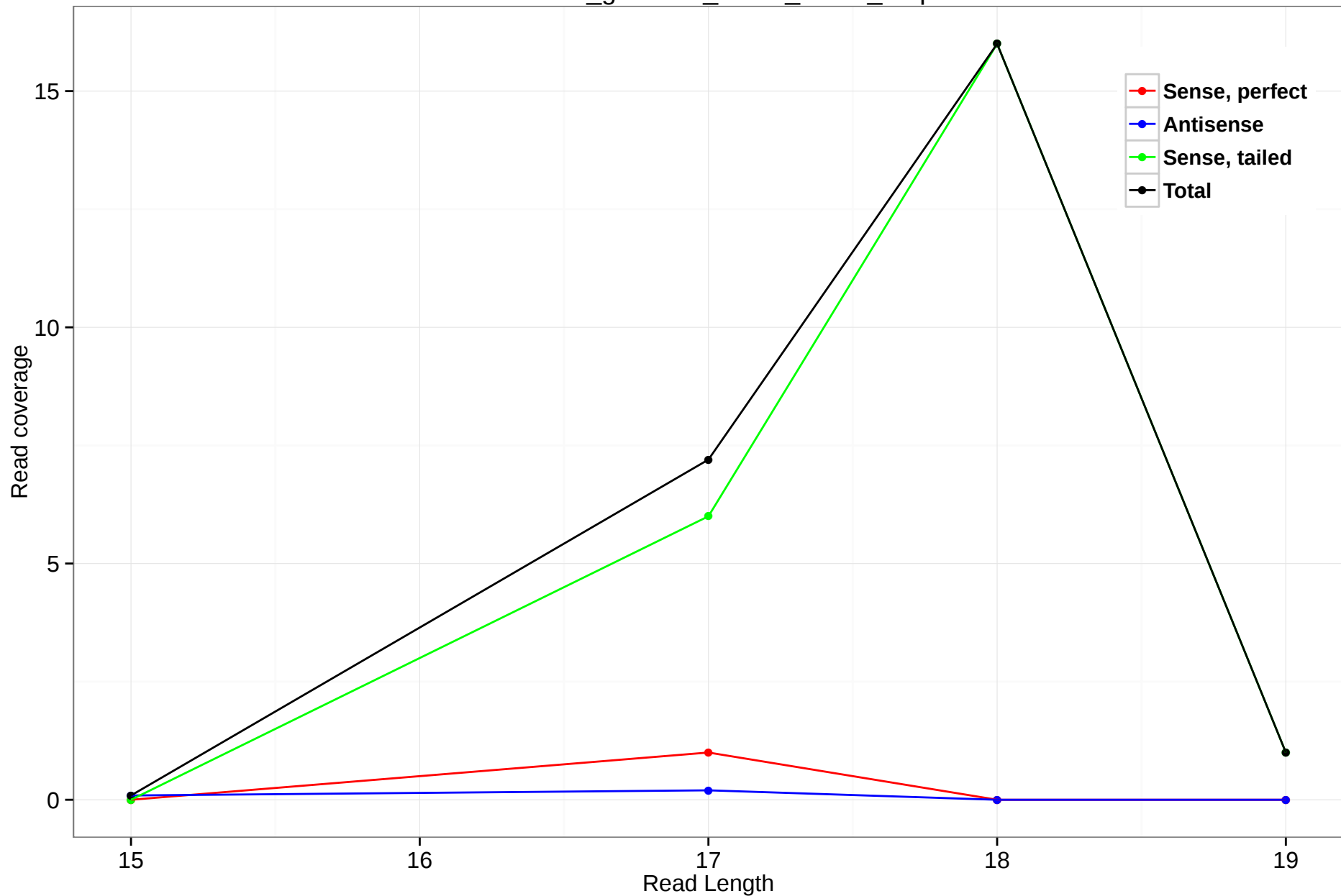
rheMac3_genscan_chr13_40.57_0.5p
