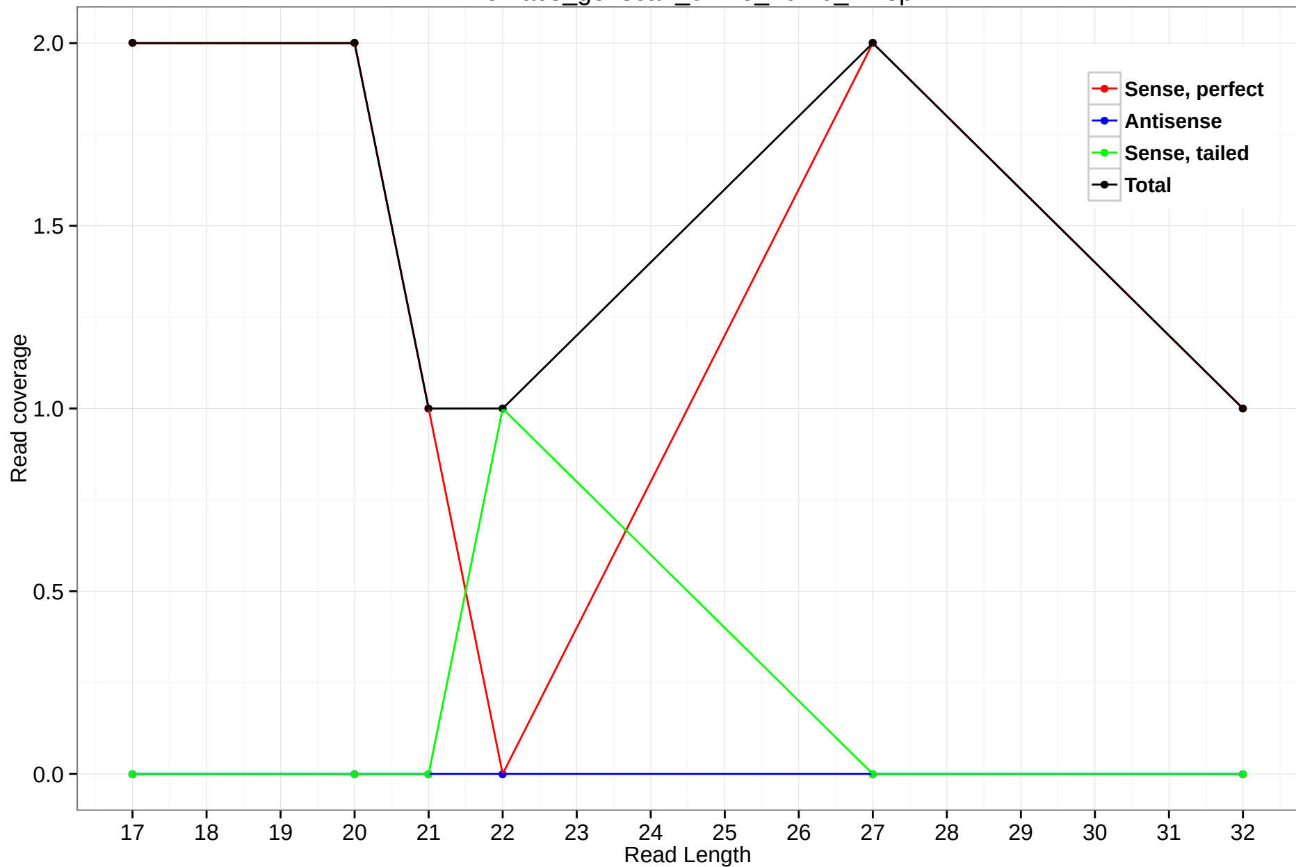
rheMac3_genscan_chr13_40.10_12.3p
