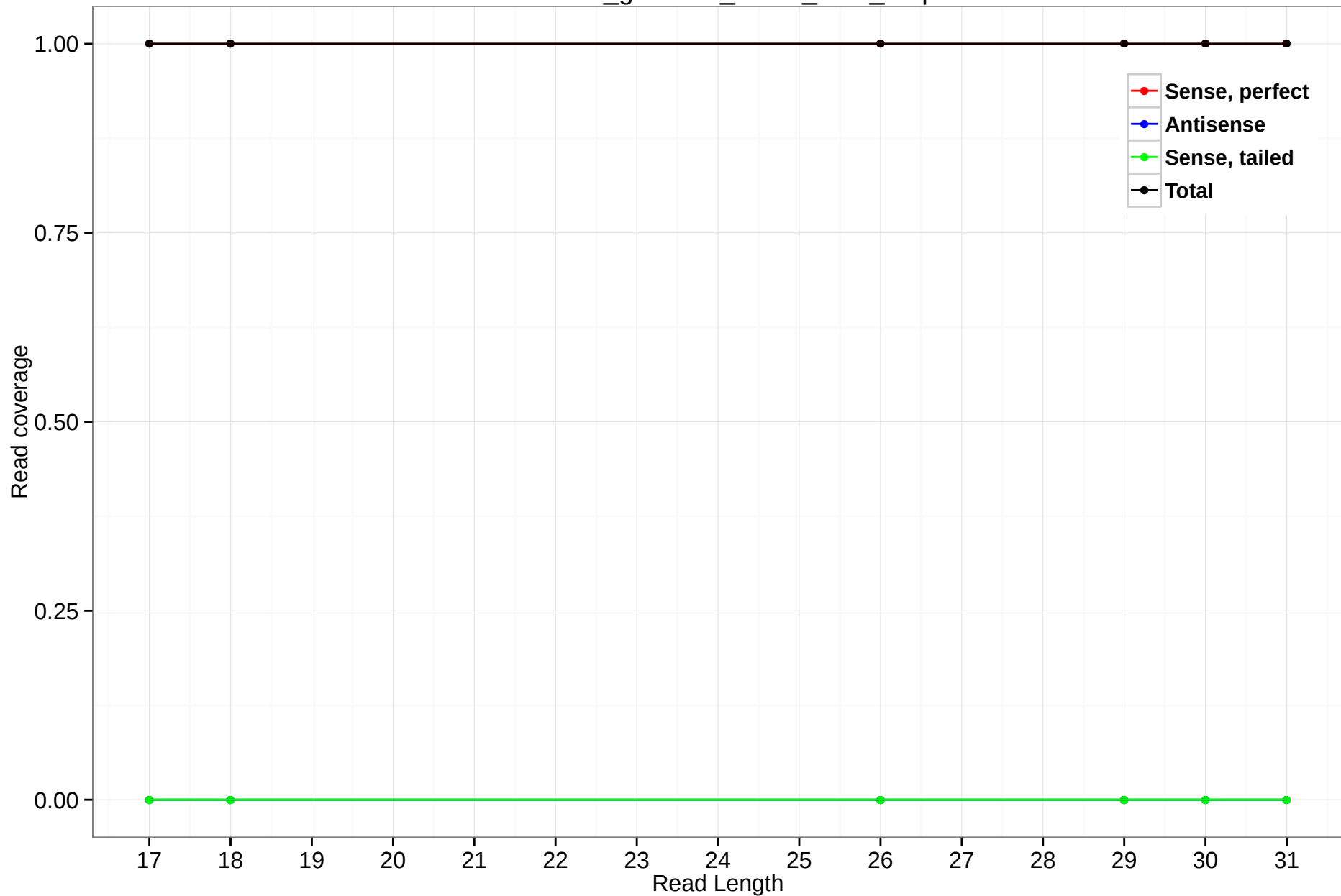
rheMac3_genscan_chr13_37.1_0.3p
