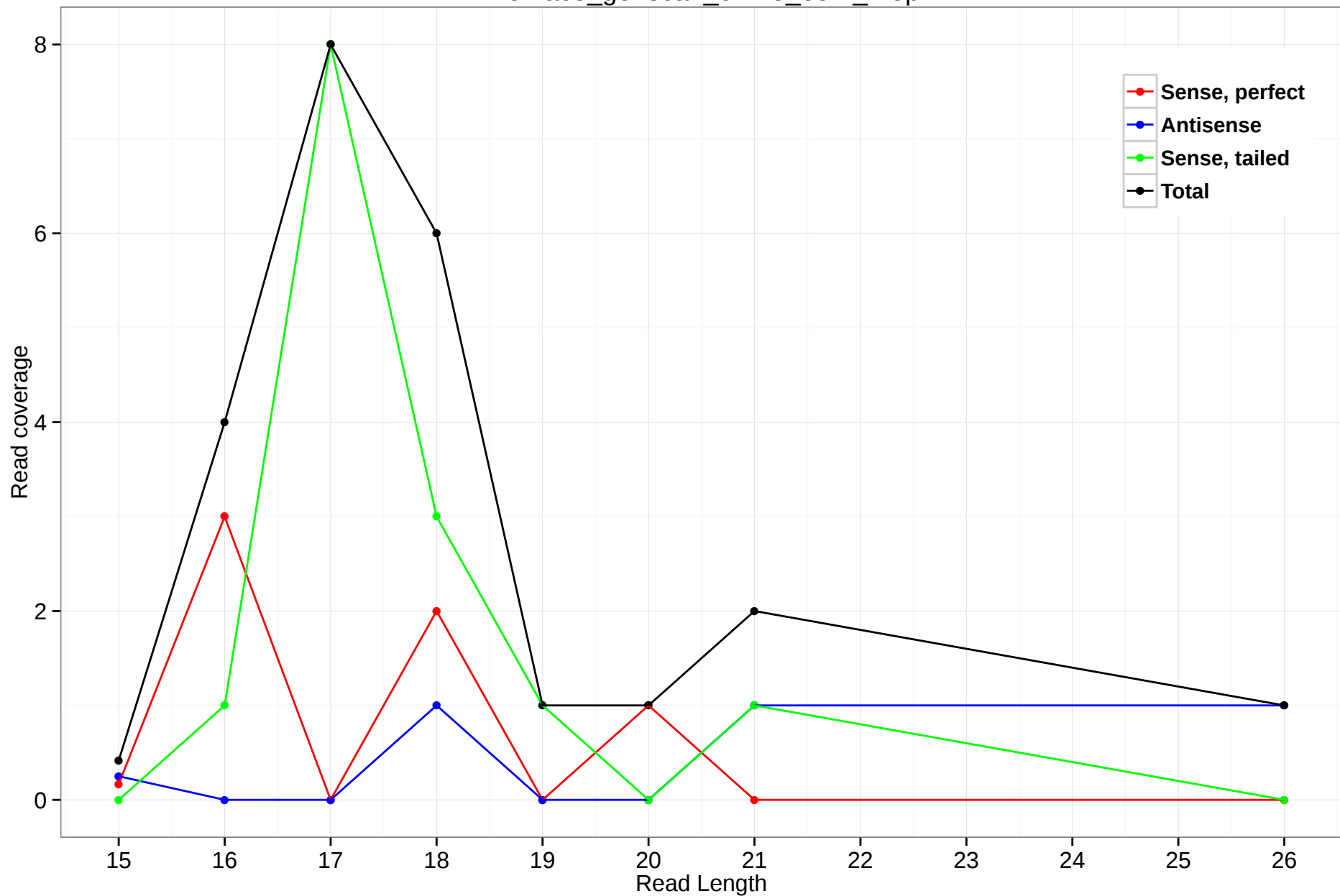
rheMac3_genscan_chr13_35.1_7.5p
