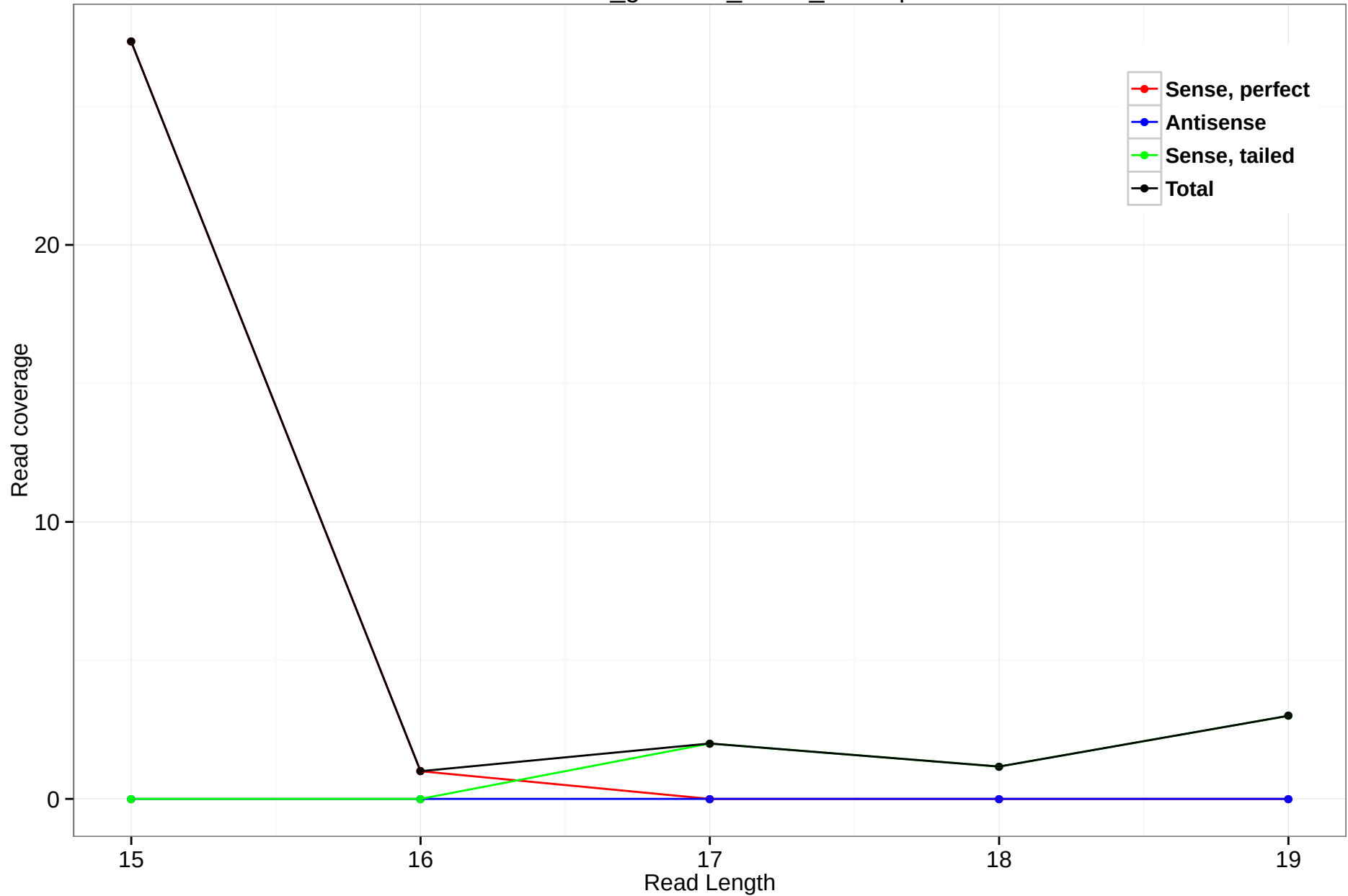
rheMac3_genscan_chr13_34.5.5p
