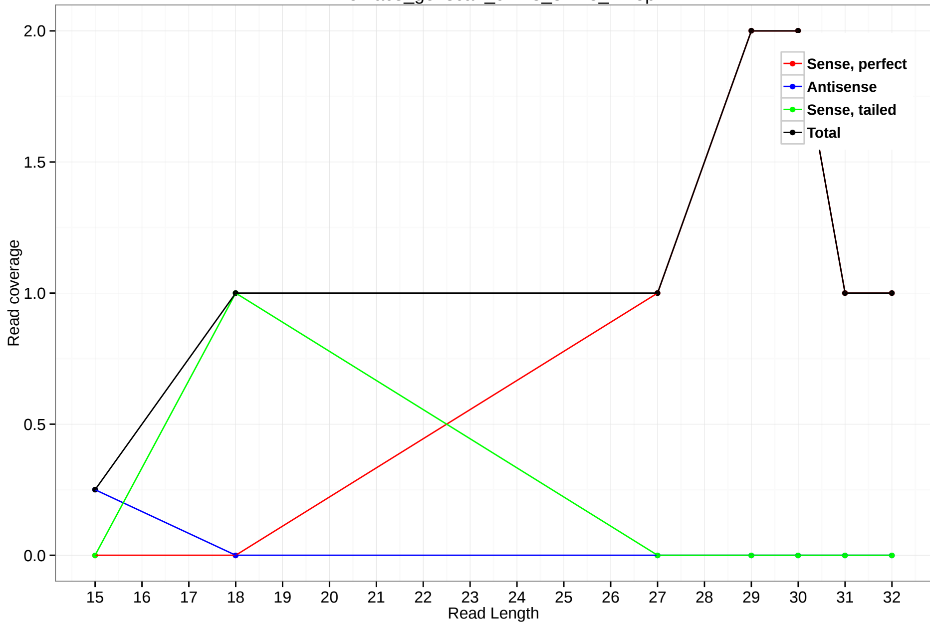
rheMac3_genscan_chr13_34.13_14.5p
