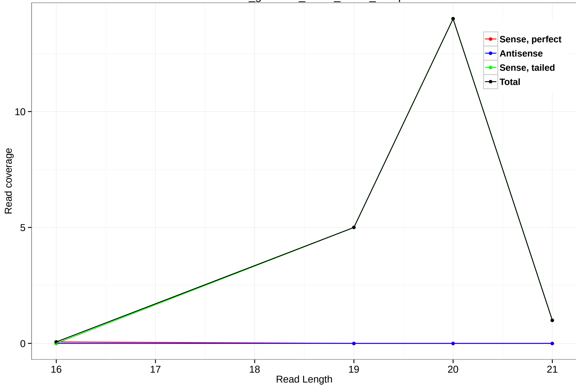
rheMac3_genscan_chr13_27.15_26.5p
