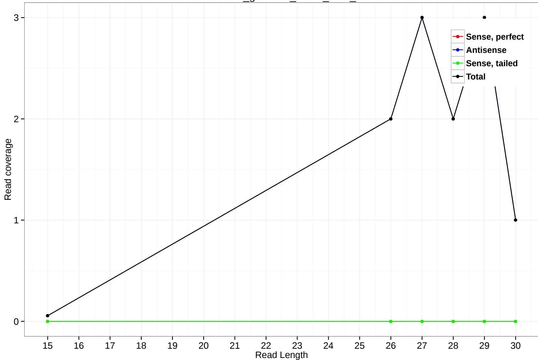
rheMac3_genscan_chr13_22.8_5
