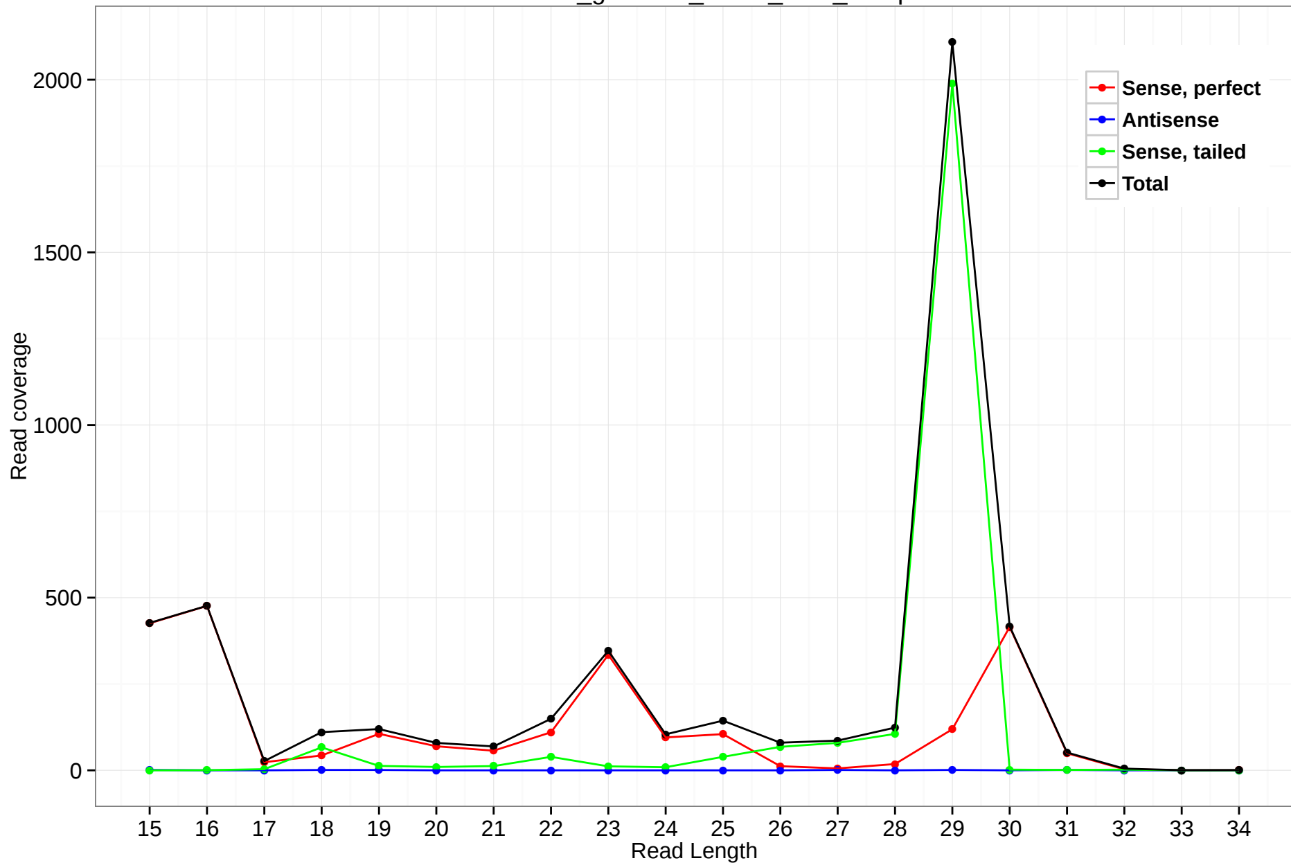
rheMac3_genscan_chr13_22.6_15.3p
