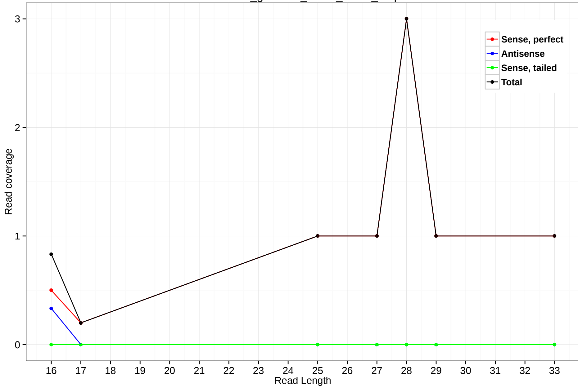
rheMac3_genscan_chr13_22.19_2.3p
