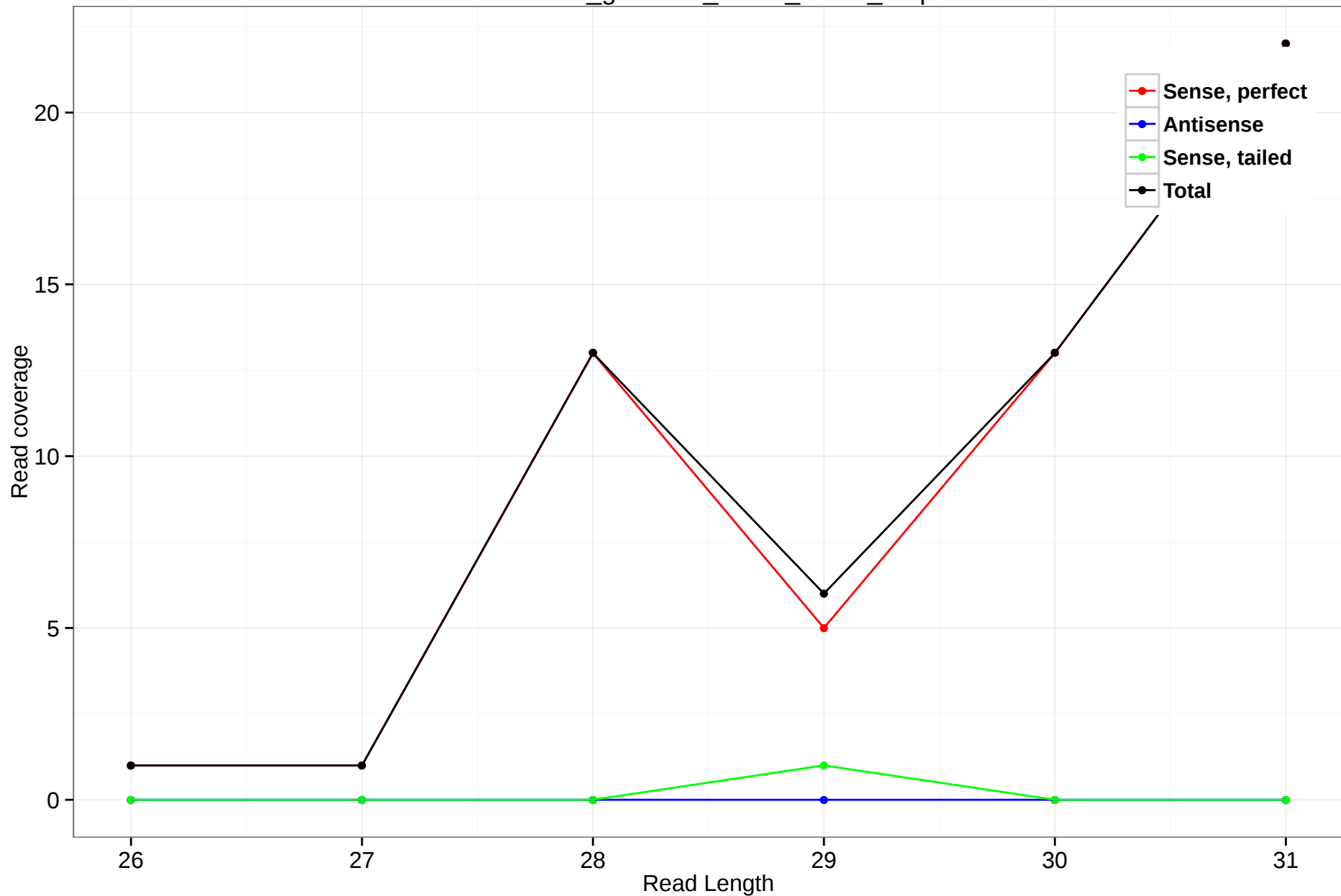
rheMac3_genscan_chr13_22.16_3.3p
