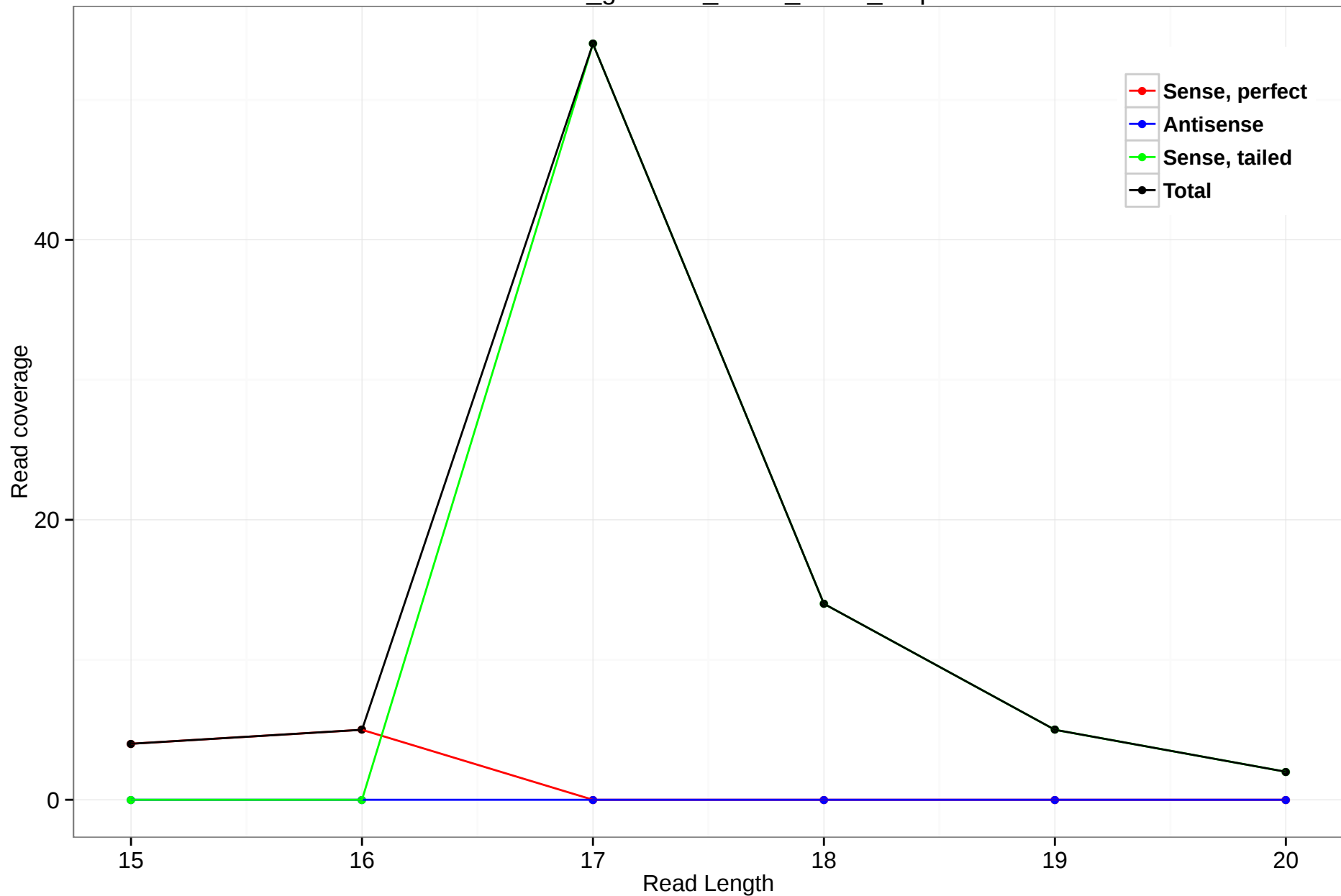
rheMac3_genscan_chr13_22.12_2.3p
