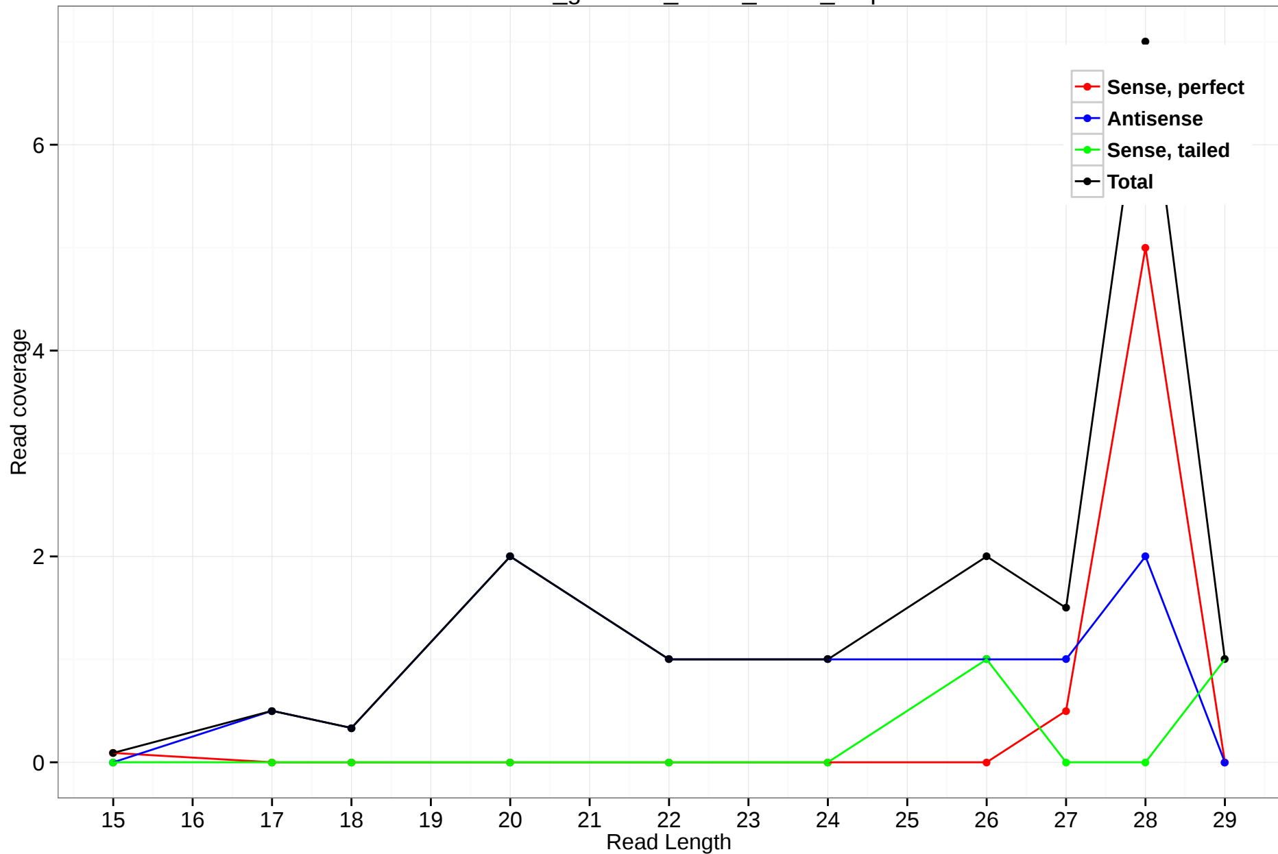
rheMac3_genscan_chr13_217.1_0.5p
