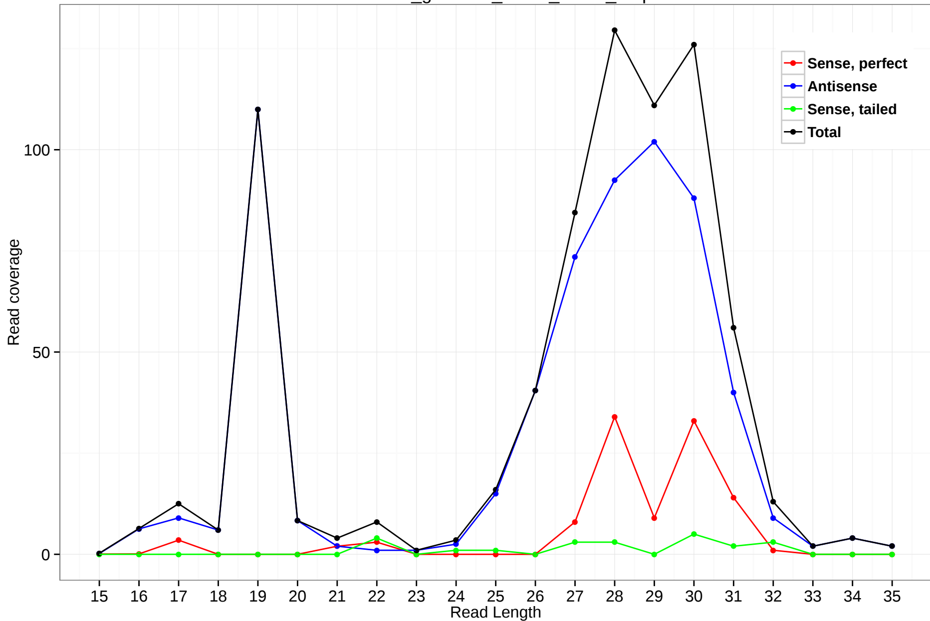
rheMac3_genscan_chr13_213.1_0.5p
