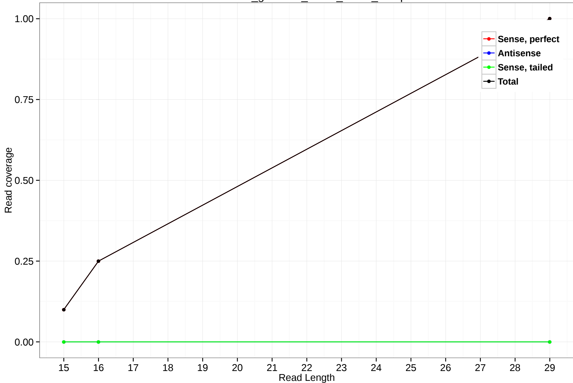
rheMac3_genscan_chr13_21.58_13.3p
