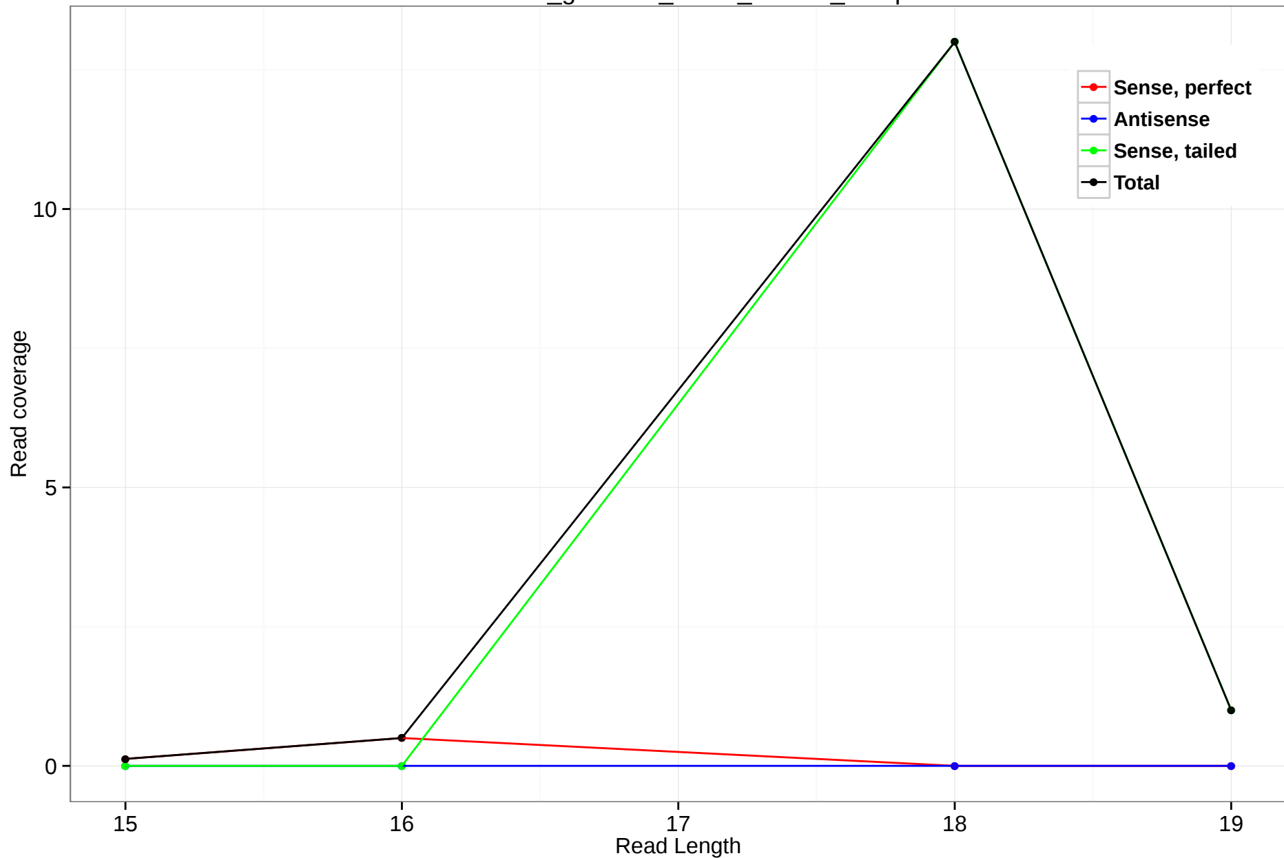
rheMac3_genscan_chr13_208.14_10.5p
