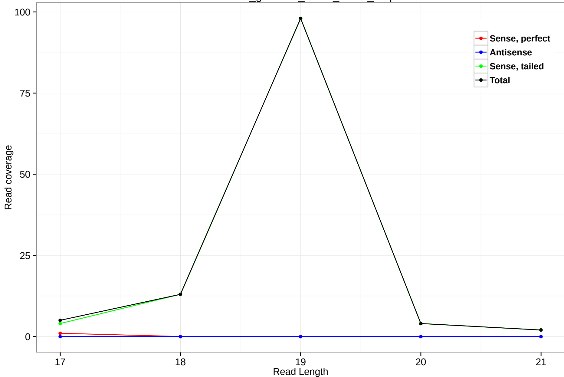
rheMac3_genscan_chr13_205.2_1.5p
