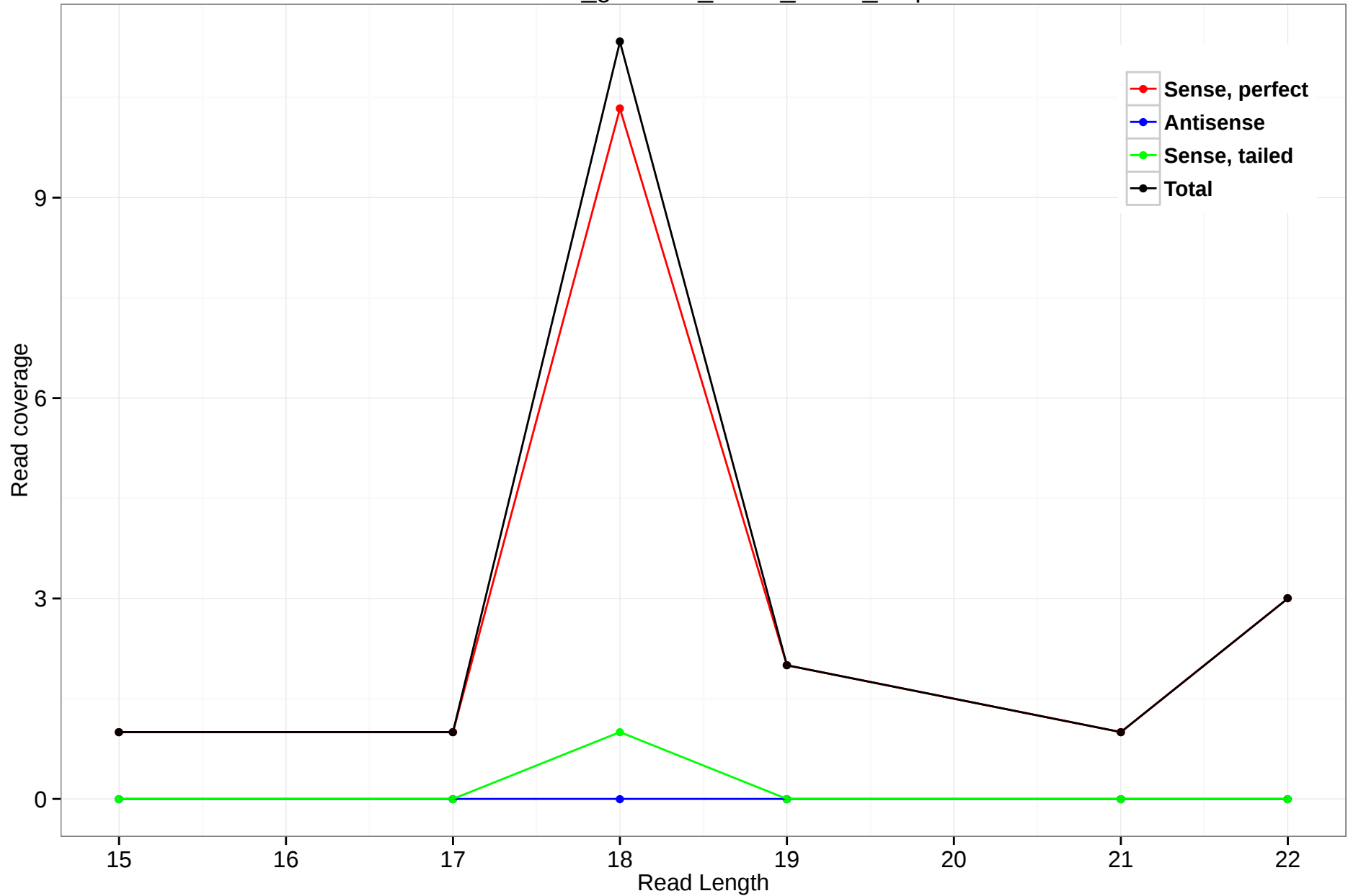
rheMac3_genscan_chr13_202.1_0.5p
