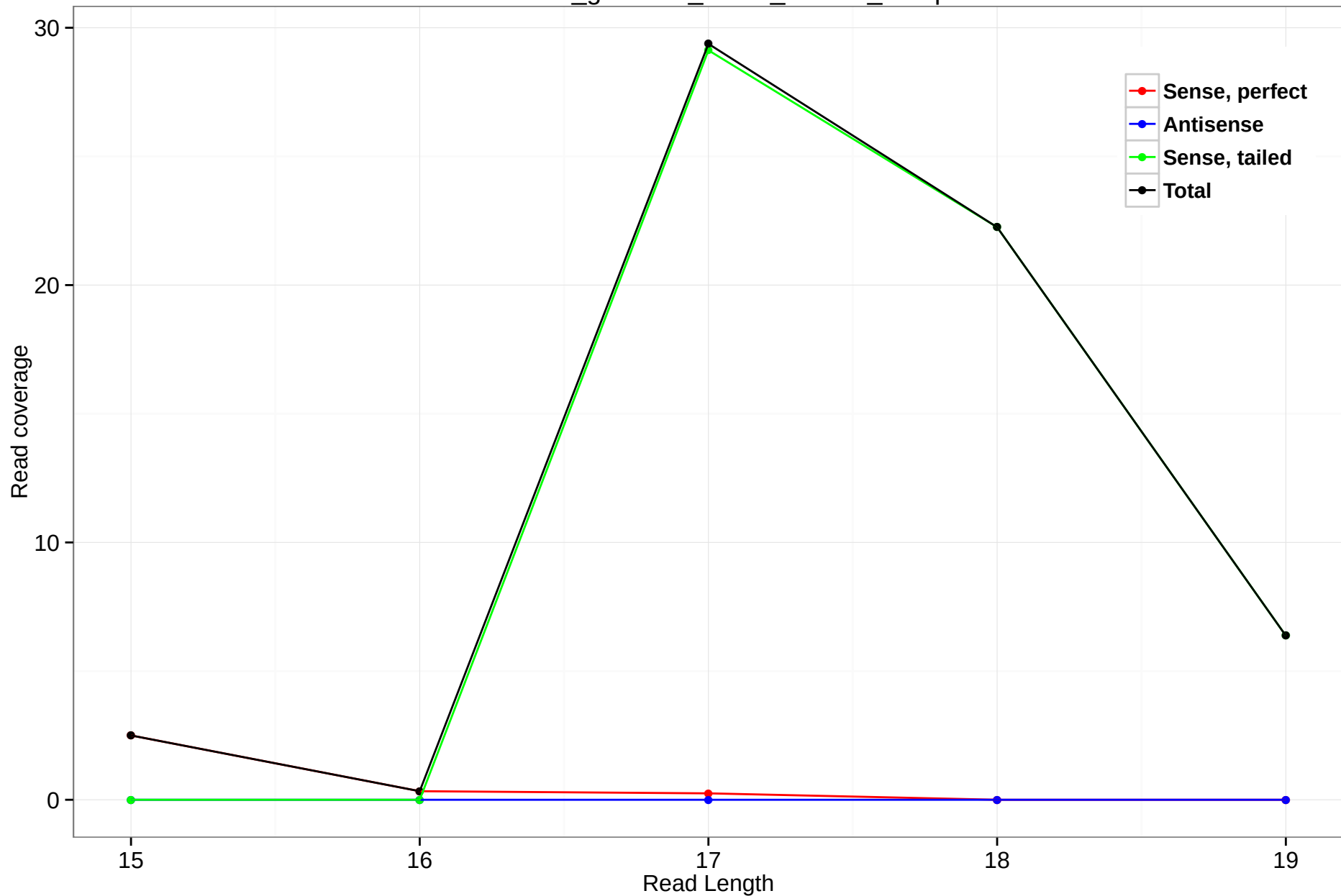
rheMac3_genscan_chr13_202.10_11.5p
