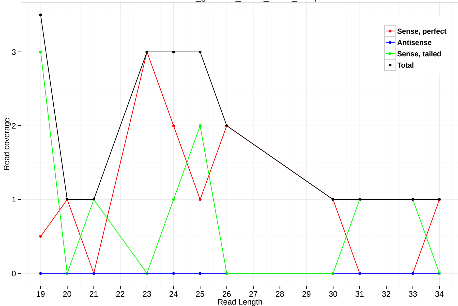
rheMac3_genscan_chr13_190.8_13.3p
