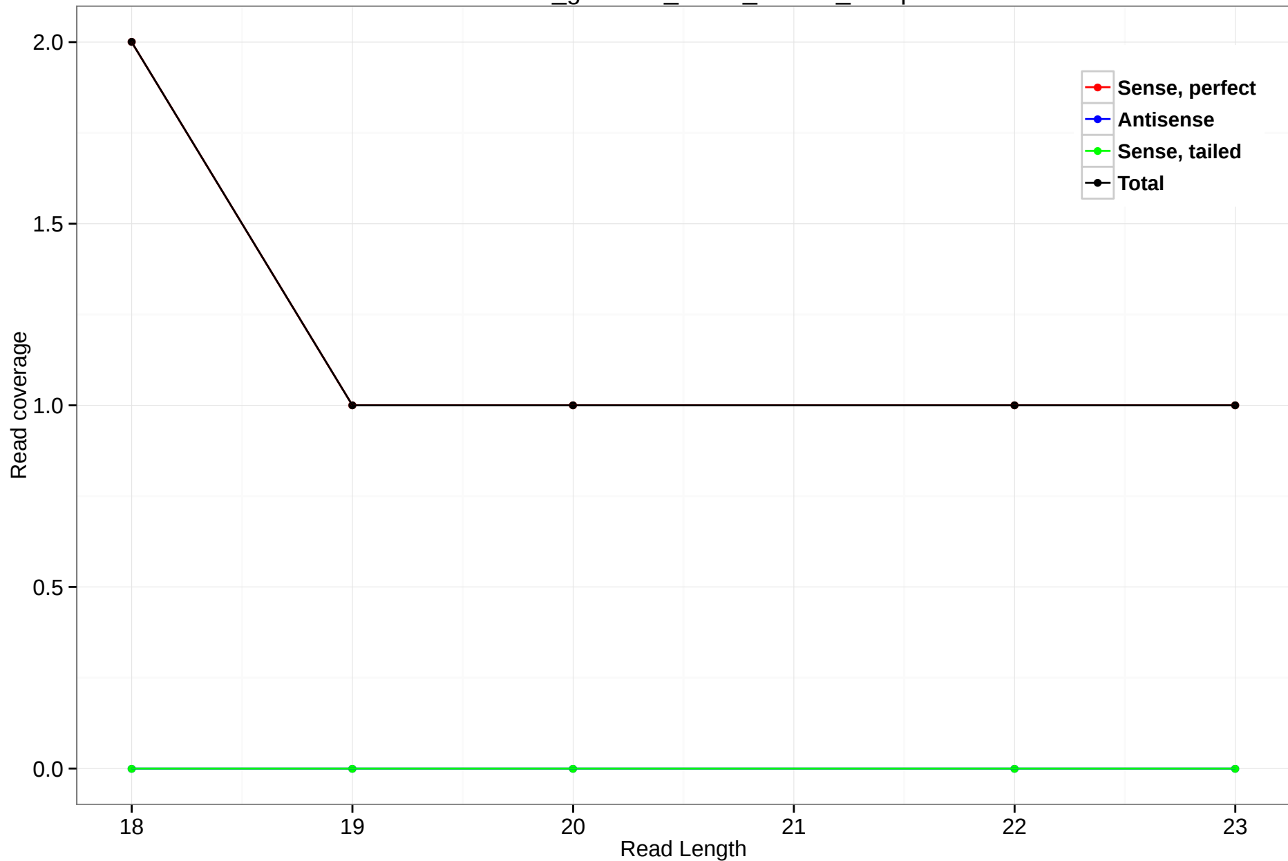
rheMac3_genscan_chr13_189.37_22.5p
