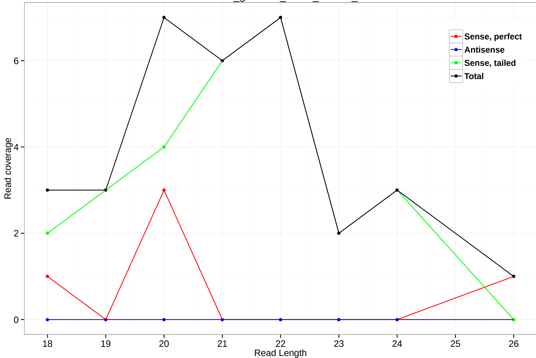
rheMac3_genscan_chr13_189.20_22
