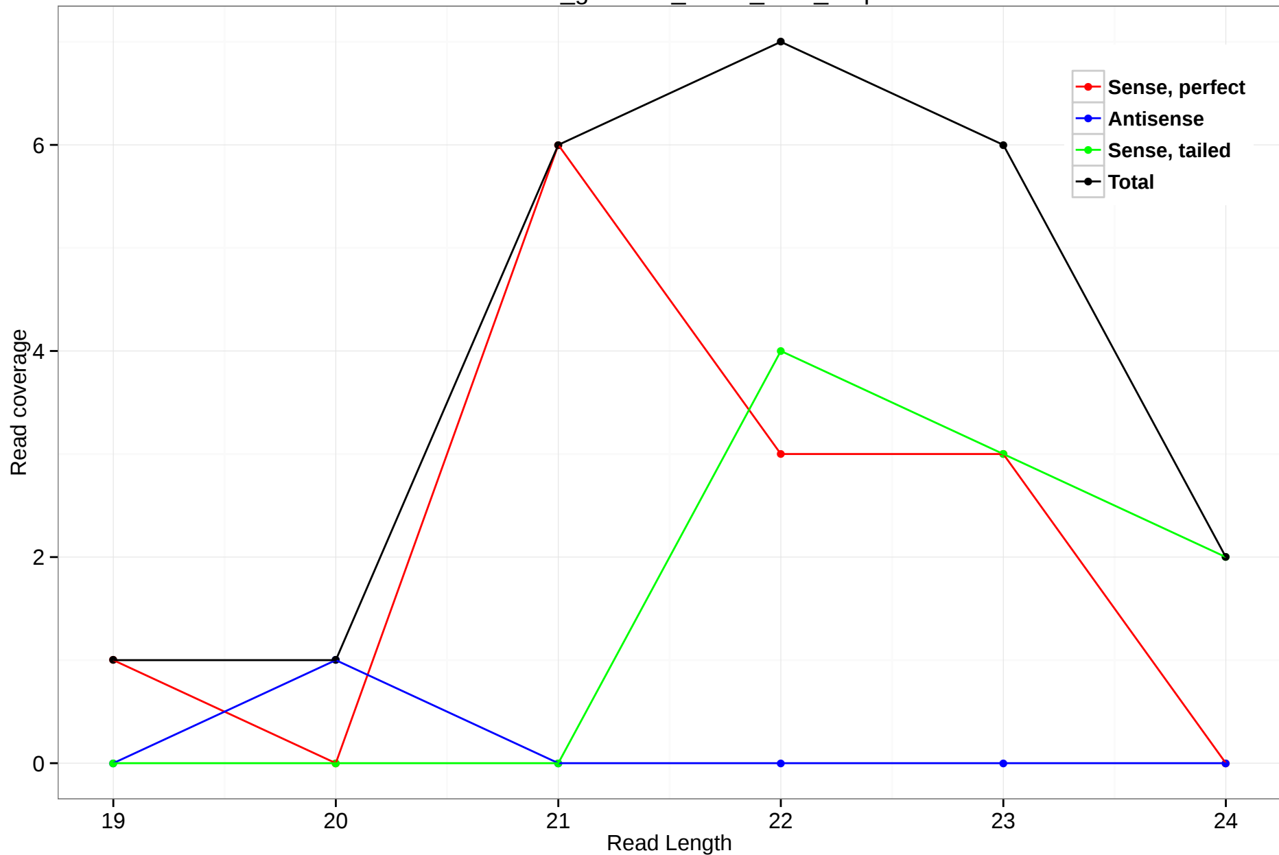
rheMac3_genscan_chr13_17.5_6.5p
