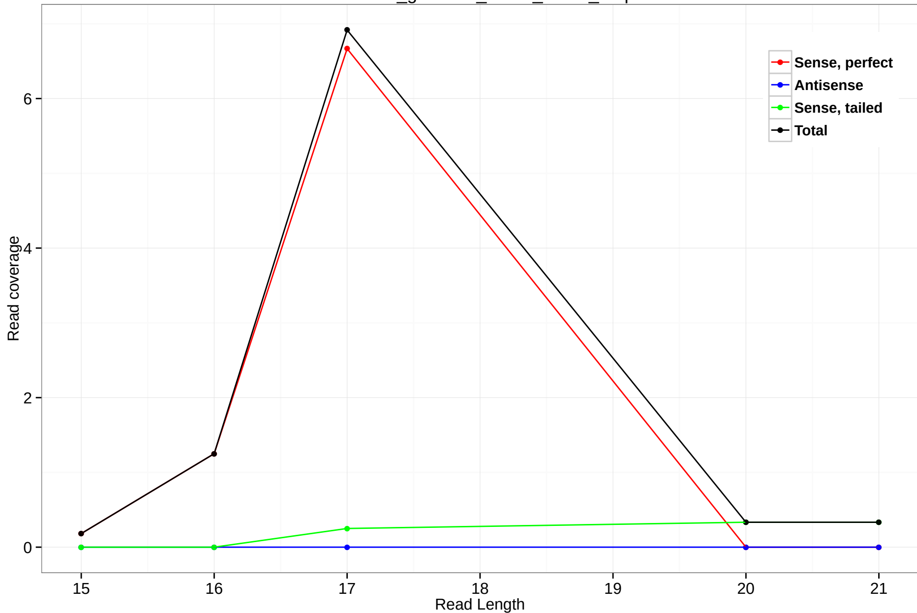
rheMac3_genscan_chr13_15.15_0.5p
