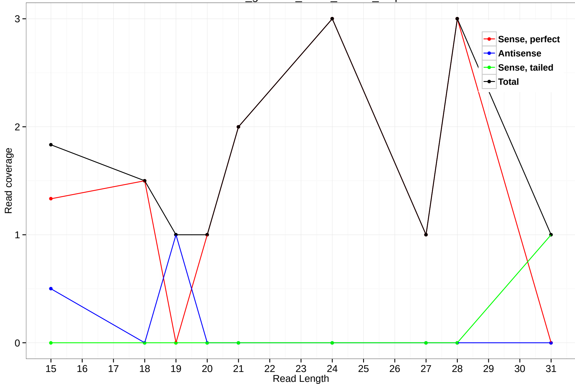
rheMac3_genscan_chr13_128.47_0.5p
