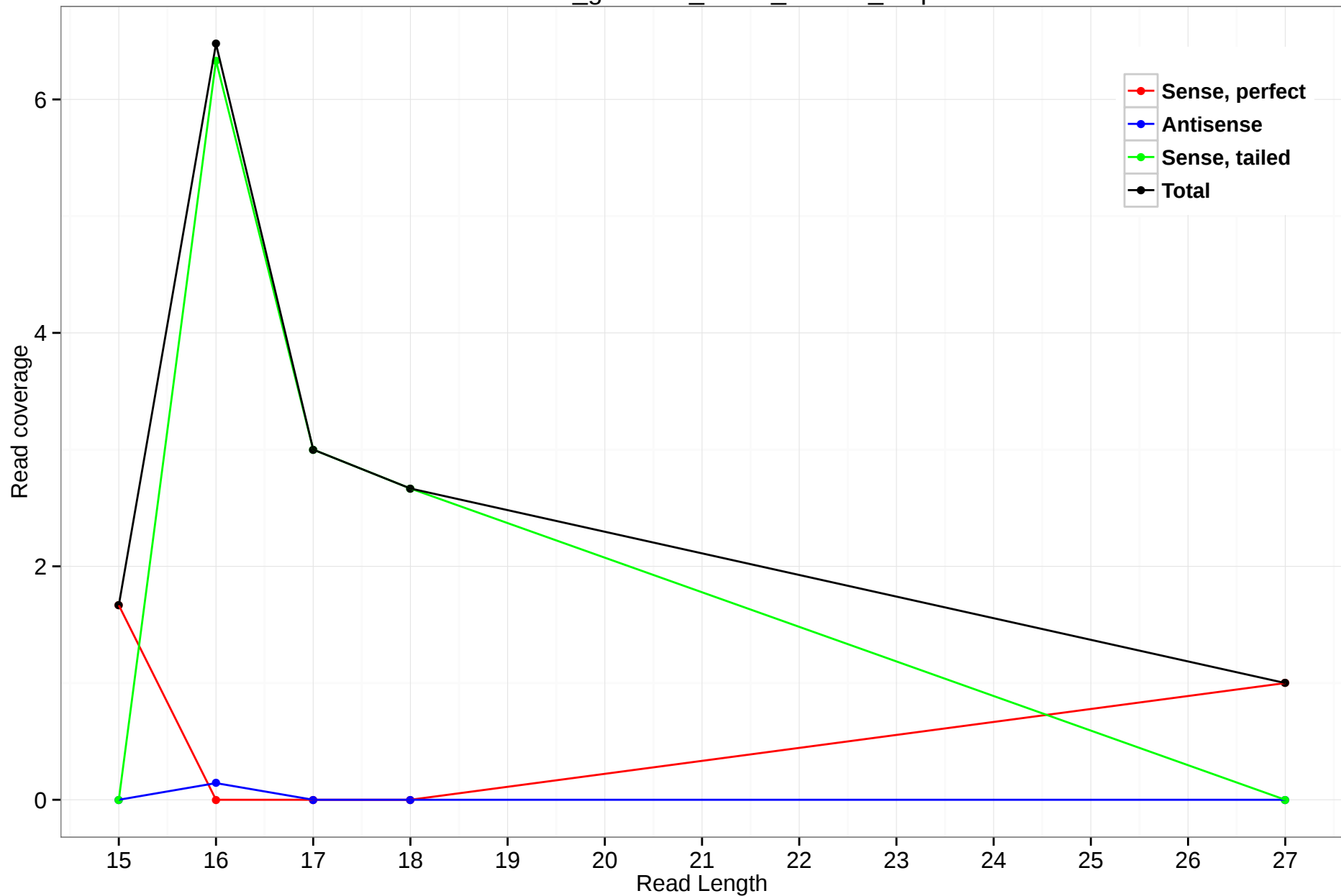
rheMac3_genscan_chr13_126.27_1.5p
