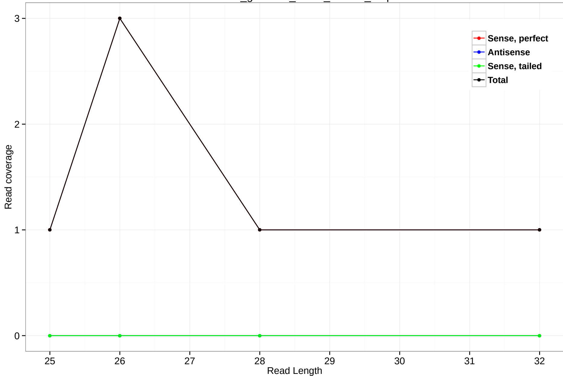
rheMac3_genscan_chr13_126.18_1.5p
