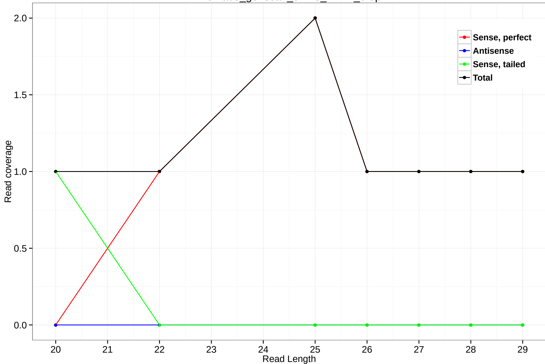
rheMac3_genscan_chr13_122.7_0.5p
