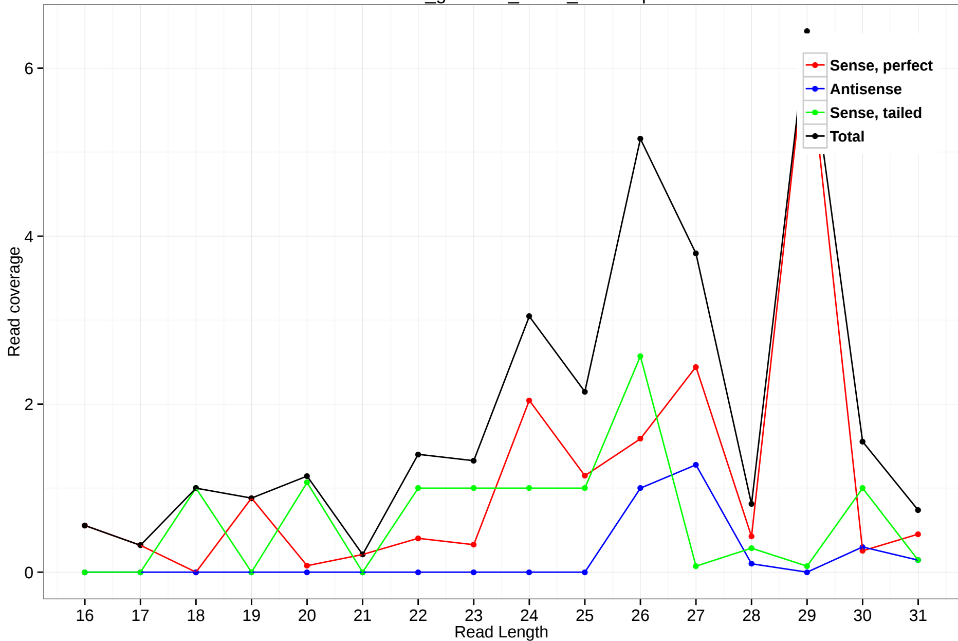
rheMac3_genscan_chr13_122.5.5p
