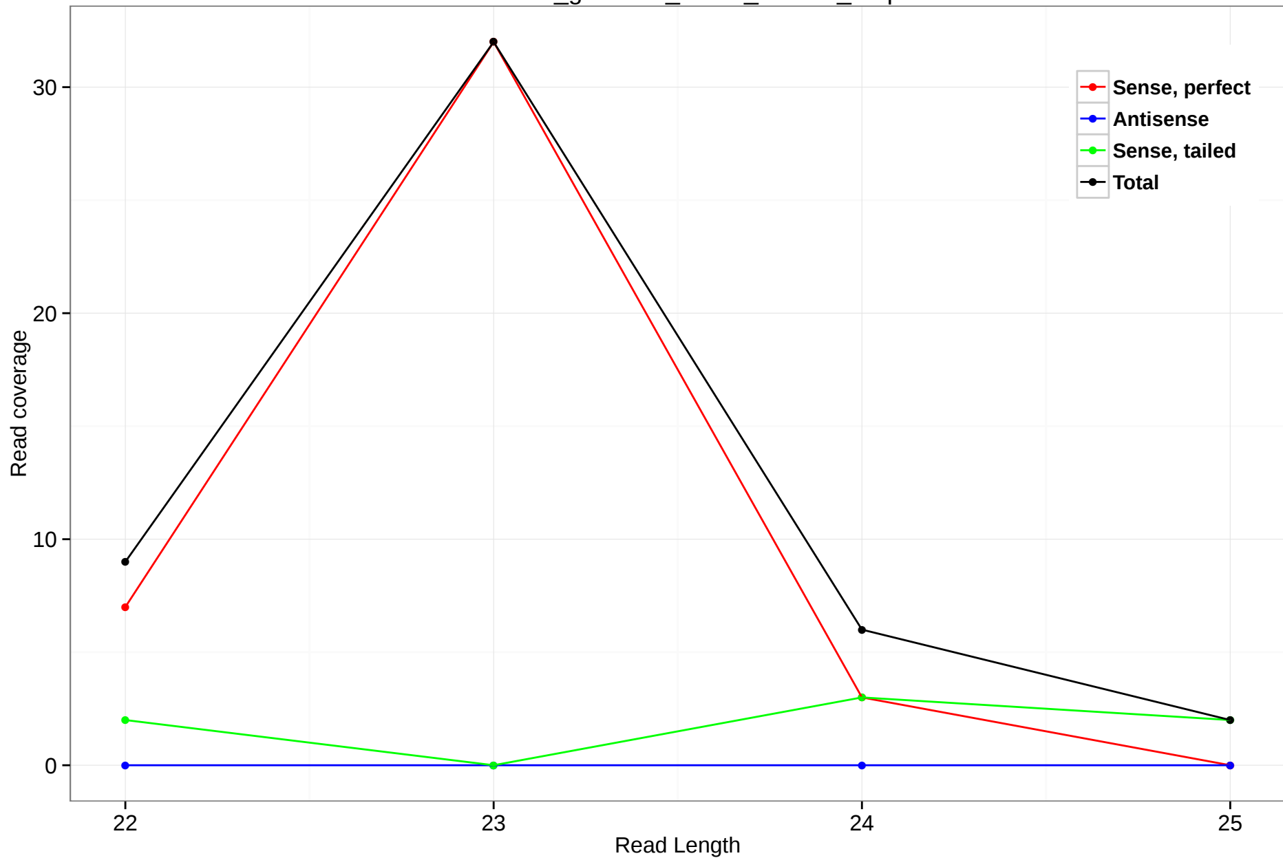
rheMac3_genscan_chr13_119.11_3.3p
