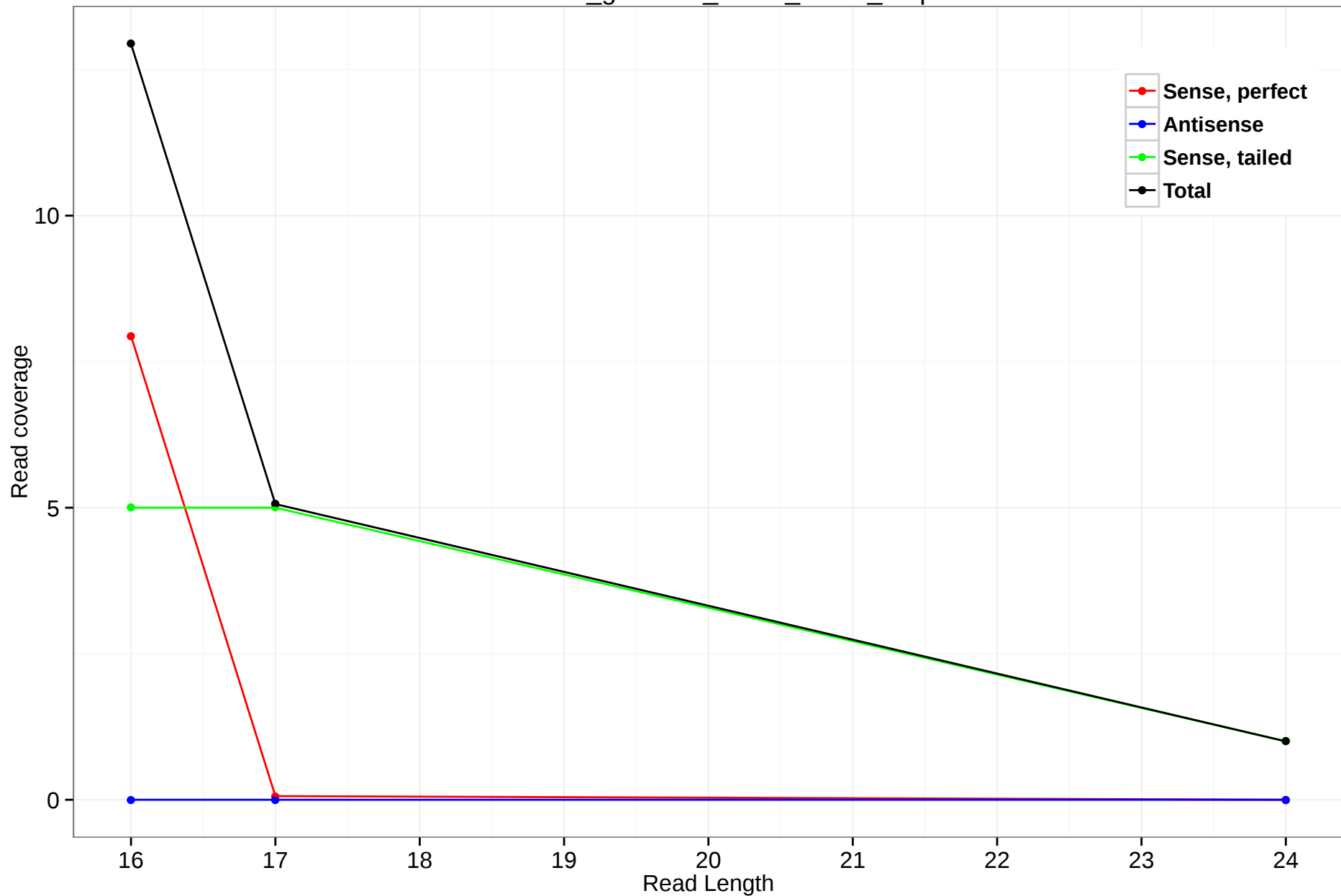
rheMac3_genscan_chr13_112.9_2.3p
