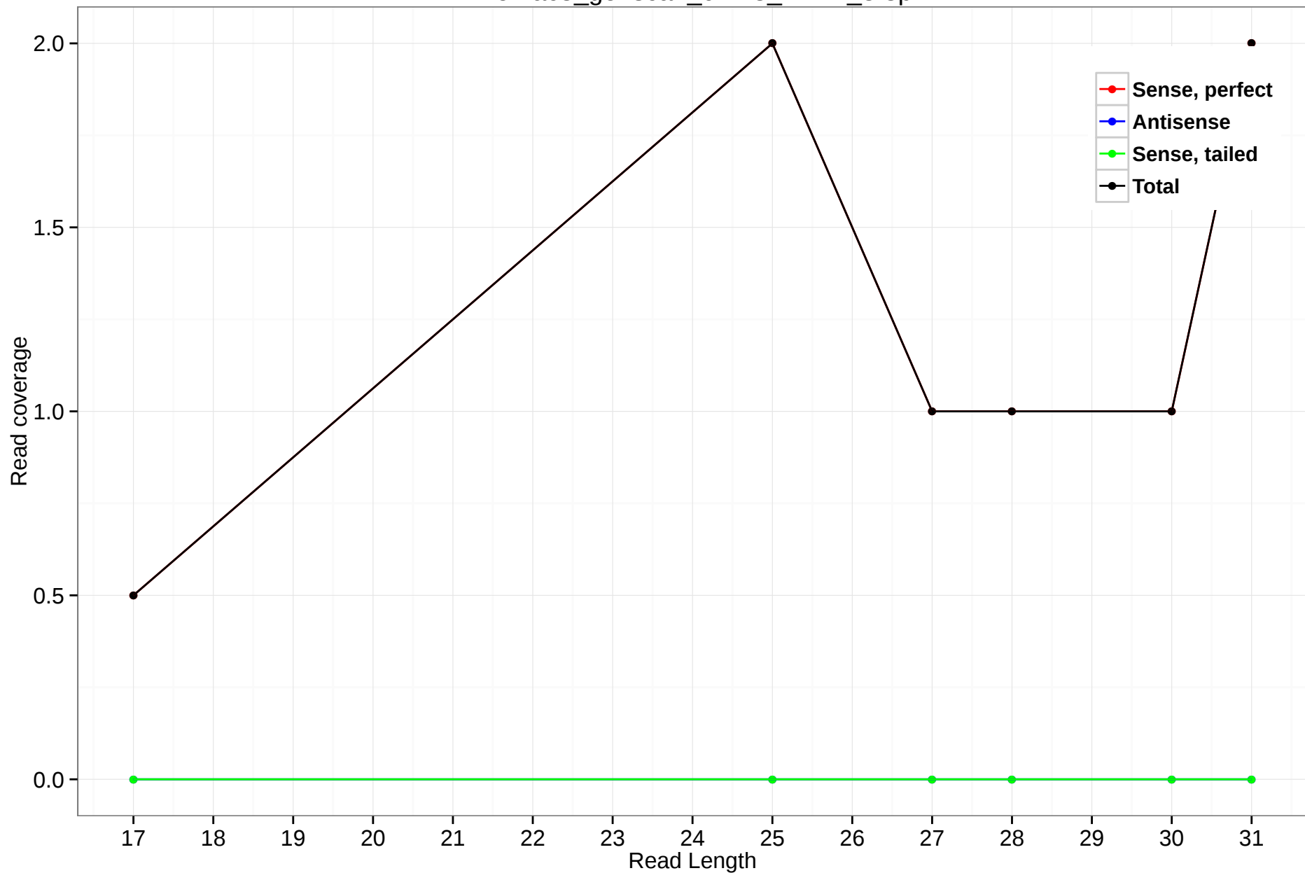
rheMac3_genscan_chr13_112.4_3.3p
