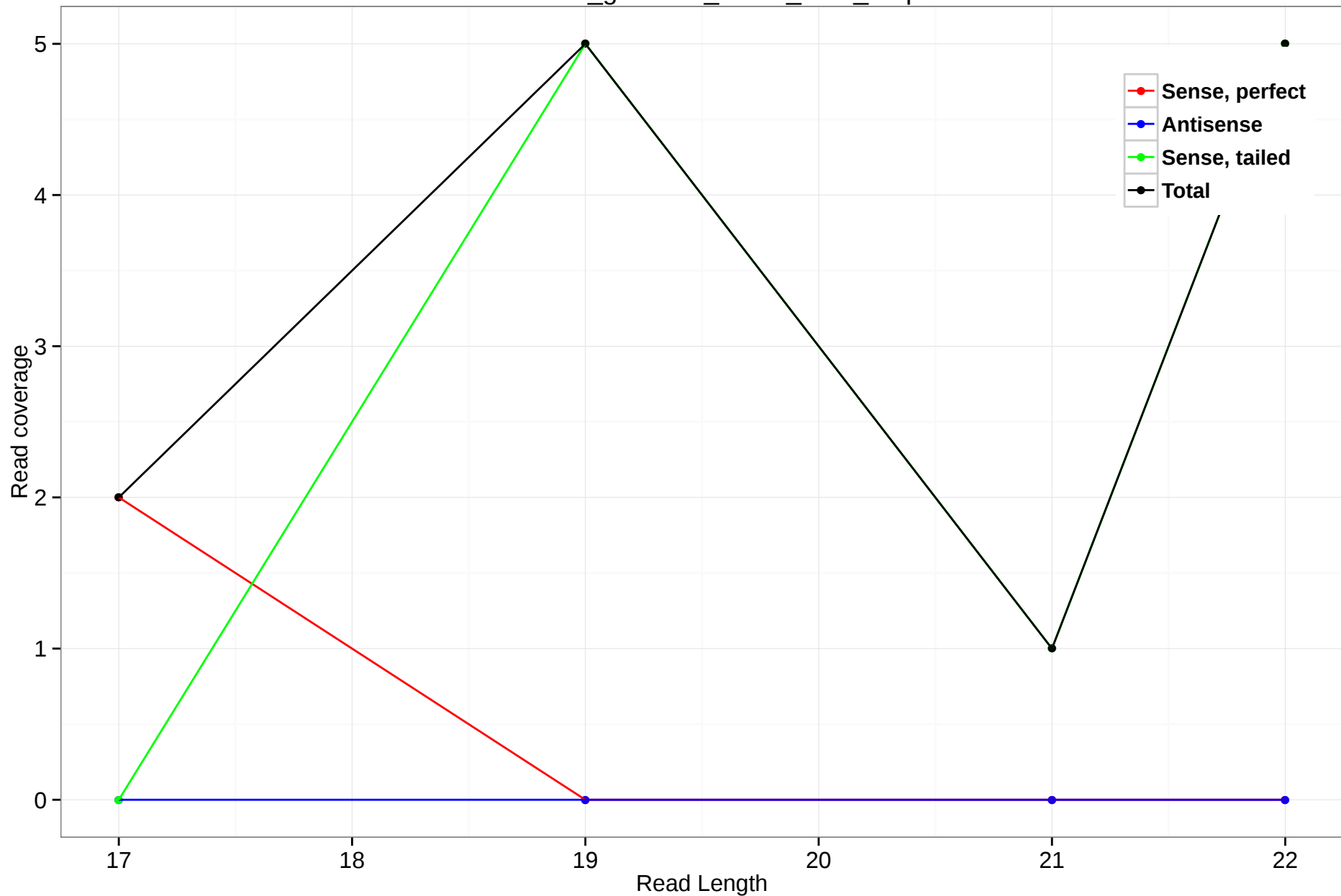
rheMac3_genscan_chr13_11.4_8.5p
