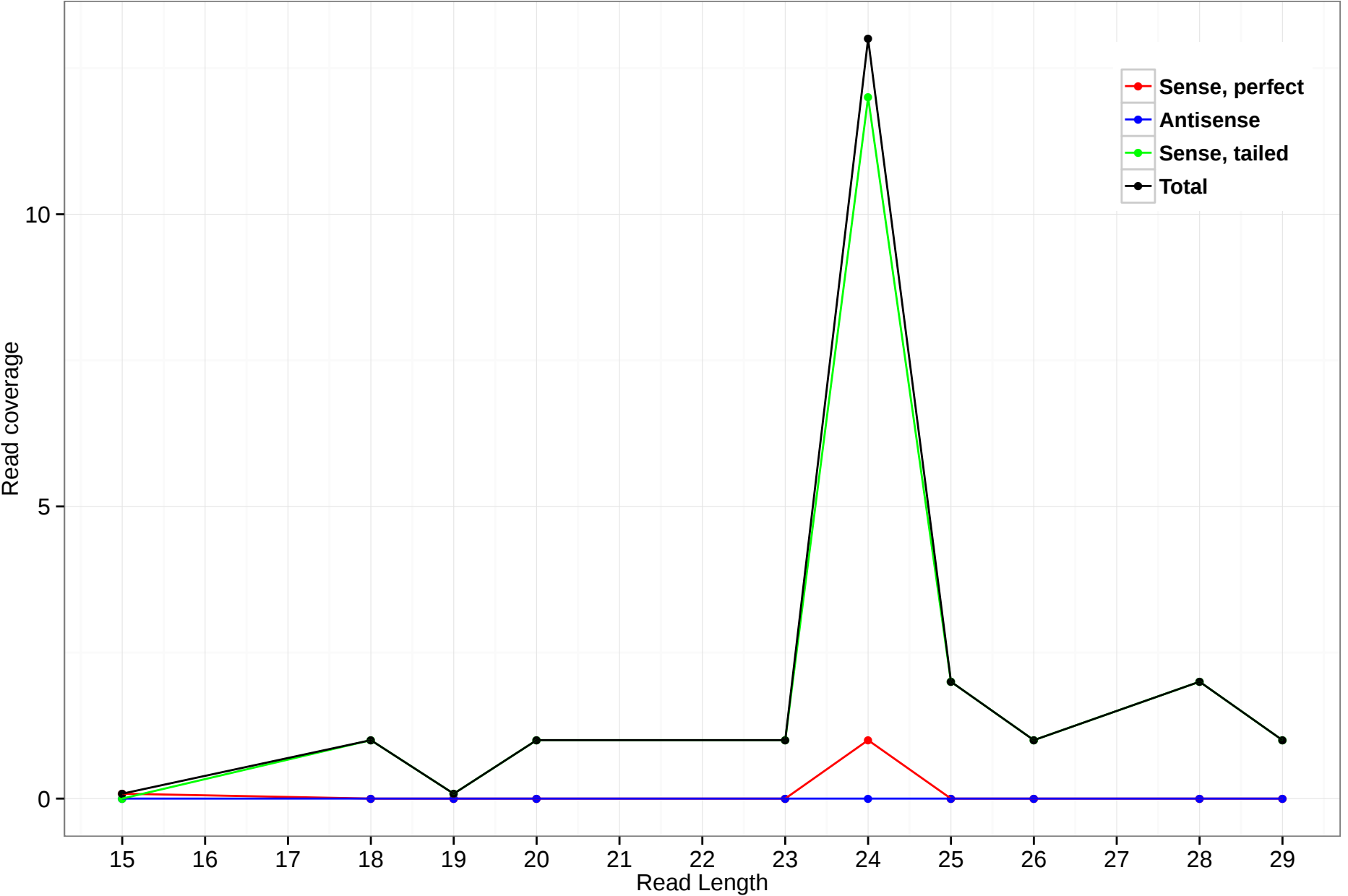
rheMac3_genscan_chr13_09.9_6
