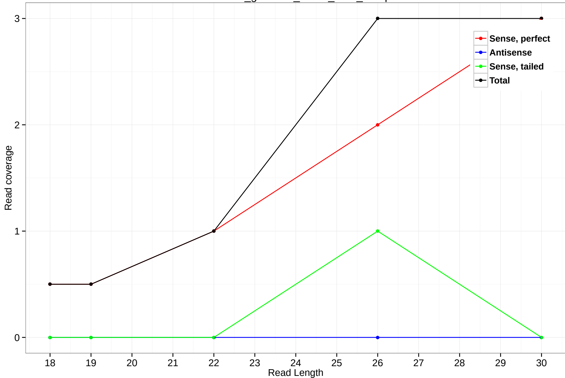
rheMac3_genscan_chr13_09.9_11.5p
